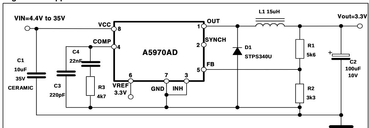
Figure 1. Application schematic
