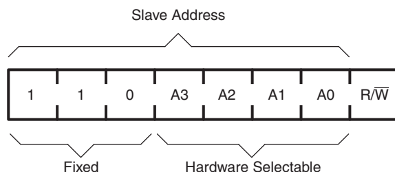
Figure 8. Slave Address
