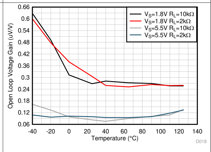
Figure 56. Open-Loop Gain vs Temperature
