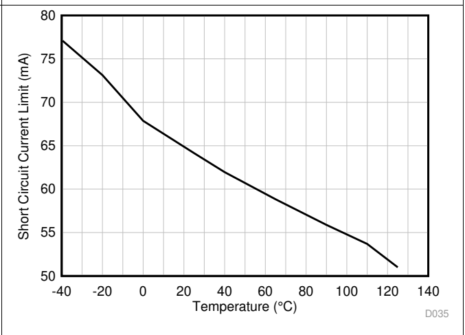
Figure 74. Short-Circuit Current vs Temperature
