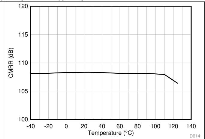
Figure 52. CMRR vs Temperature
