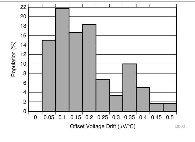
Figure 40. Offset Voltage Drift Distribution
