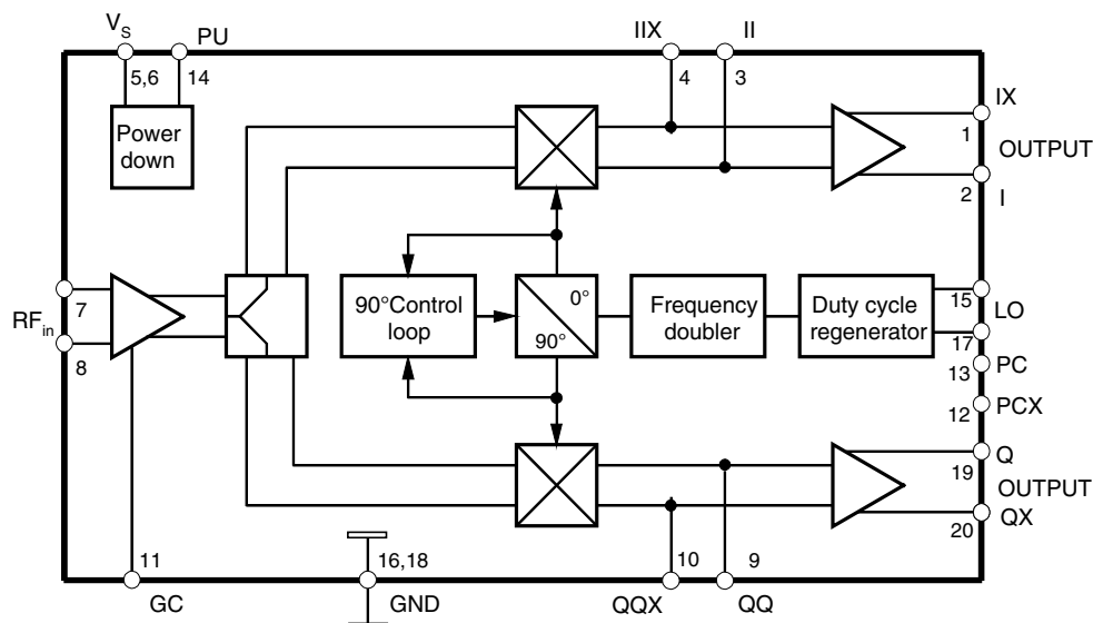
Figure 1-1. Block Diagram
