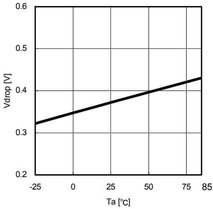
Fig.16 Minimum dropout Voltage (Vcc=5V, Io=-0.3A)
