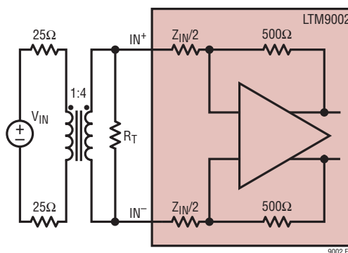
Figure 5. Input Termination for Differential 50\Omega Input Impedance Using a Balun
