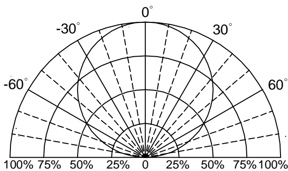
Fig.5 Directive Radiation
