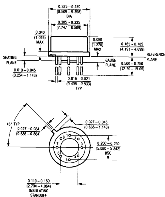
H Package 8 Lead TO-5 Metal Can
