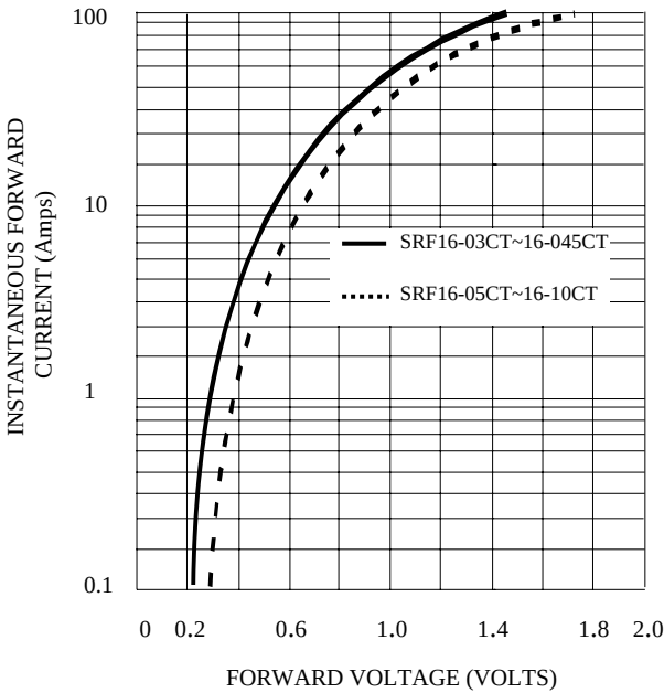
FIG. 5 - TYPICAL FORWARD CHARACTERISTIC
