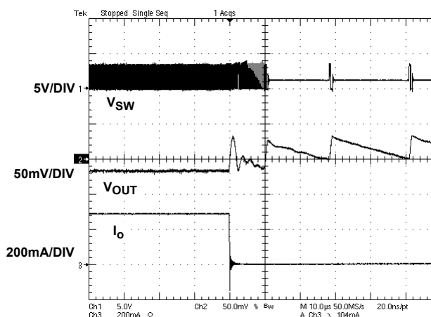
FIGURE 14. LOAD TRANSIENT FROM PWM TO PFM MODE ( V_{IN} = 3.6V , V_{OUT} = 1.5V , 300mA TO 5mA)
