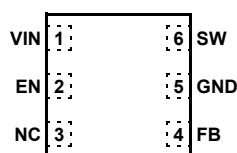
ISL9103, ISL9103A (6 LD 1.6x1.6 UTDFN) TOP VIEW
