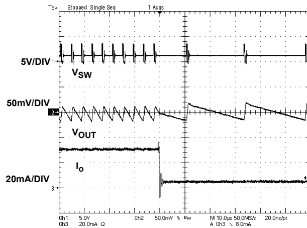
FIGURE 10. LOAD TRANSIENT IN PFM MODE ( V_{IN} = 3.6V , V_{OUT} = 1.5V , 30mA TO 5mA)
