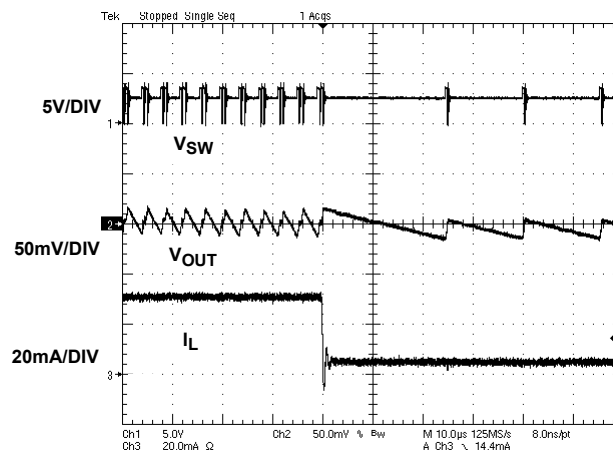
FIGURE 12. LOAD TRANSIENT IN PFM MODE ( V_{IN} = 3.6V , V_{OUT} = 2.5V , 30mA TO 5mA)
