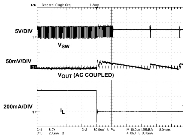
FIGURE 16. LOAD TRANSIENT FROM PWM TO PFM MODE ( V_{IN} = 3.6V , V_{OUT} = 2.5V , 300mA TO 5mA)
