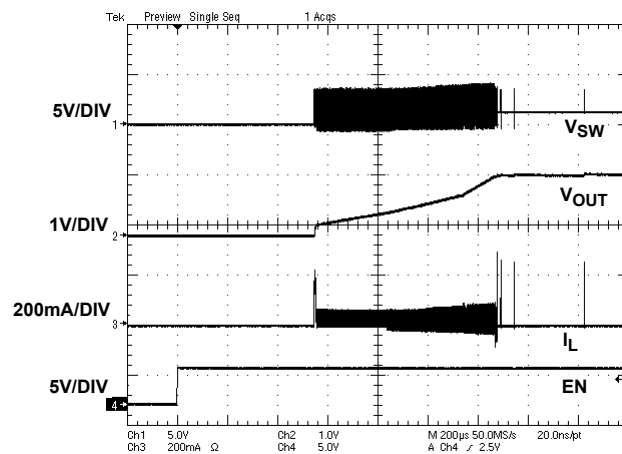
FIGURE 6. SOFT-START TO PFM MODE ( V_{IN} = 3.6V , V_{OUT} = 1.5V , I_{OUT} = 0.001mA )
