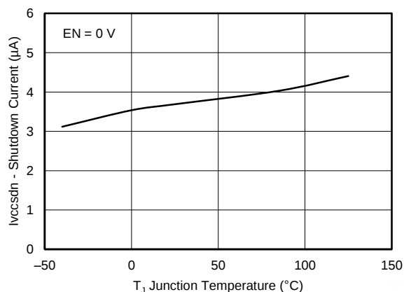
Figure 2. SHUTDOWN CURRENT vs JUNCTION TEMPERATURE
