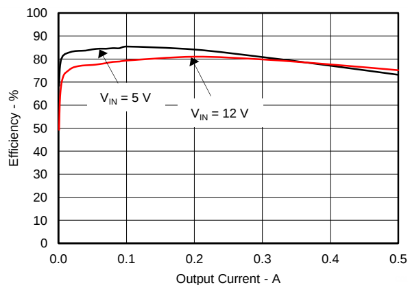
Figure 8. Efficiency
