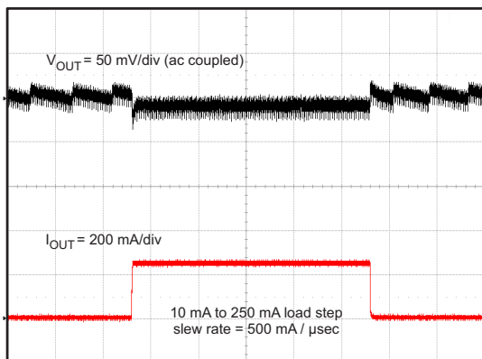
Figure 14. Transient Response, 2% to 50% Load Step
