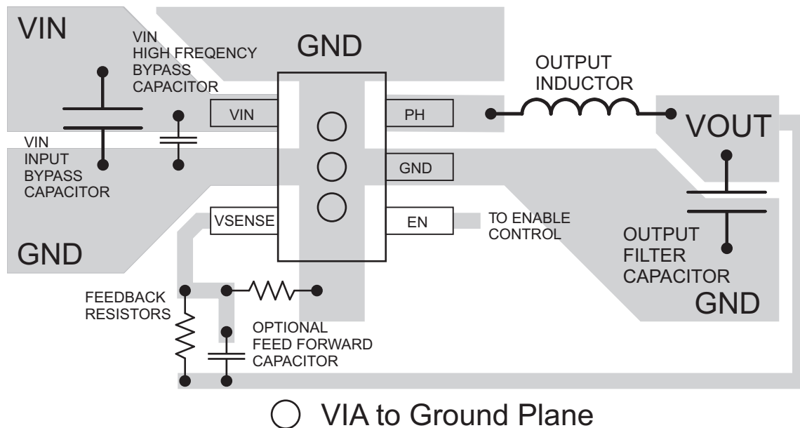
Figure 19. Typical Layout
