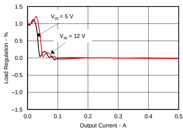
Figure 10. Load Regulation
