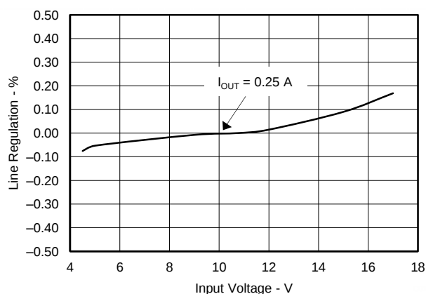
Figure 11. Line Regulation
