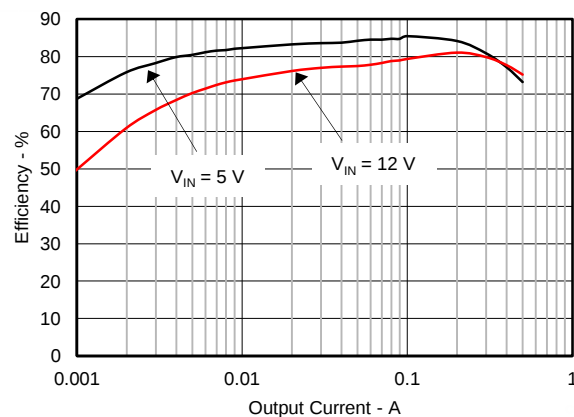
Figure 9. Light Load Efficiency
