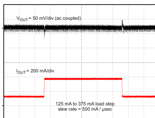
Figure 13. Transient Response, 25% to 75% Load Step
