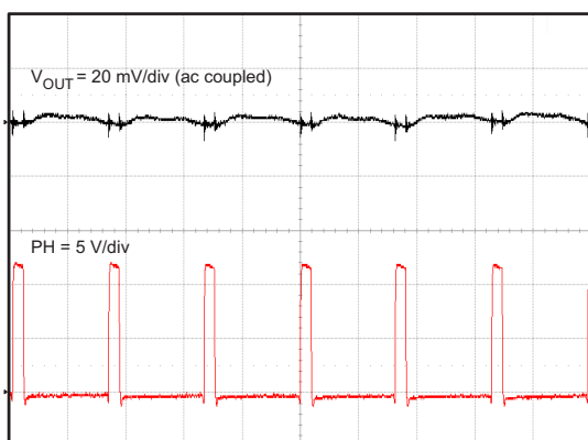
Figure 16. Output Ripple, I_{OUT} = 500\text{ mA}
