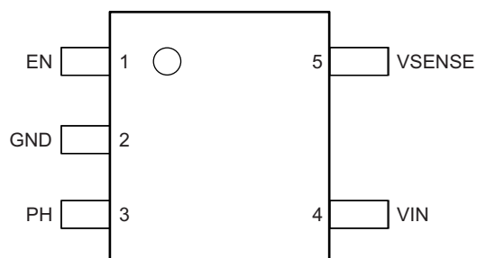
SOT23 PACKAGE (TOP VIEW)
