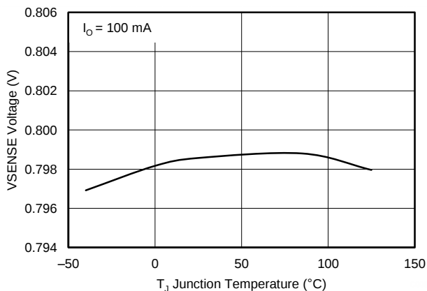
Figure 6. VSENSE VOLTAGE vs JUNCTION TEMPERATURE
