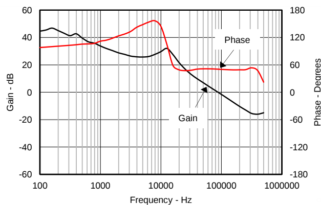
Figure 12. Loop Response, I_{OUT} = 0.25\text{ A}
