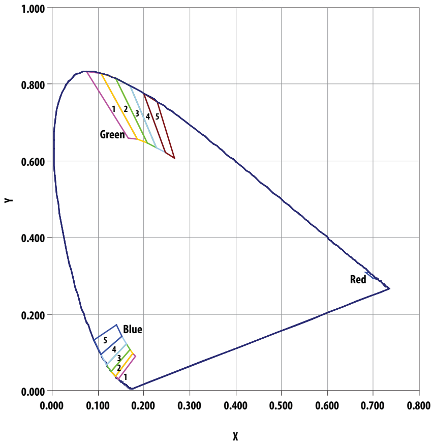
CIE 1931 - Chromaticity Diagram
