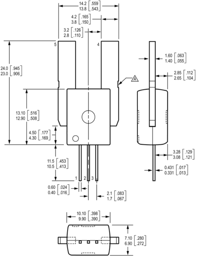
Package CB-PSS
