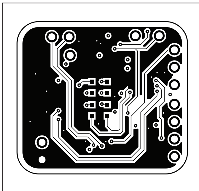
MAX30110 EV Kit—Top
