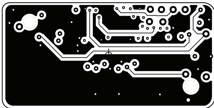
MAX30110 EV Kit—Level 4 SIGS
