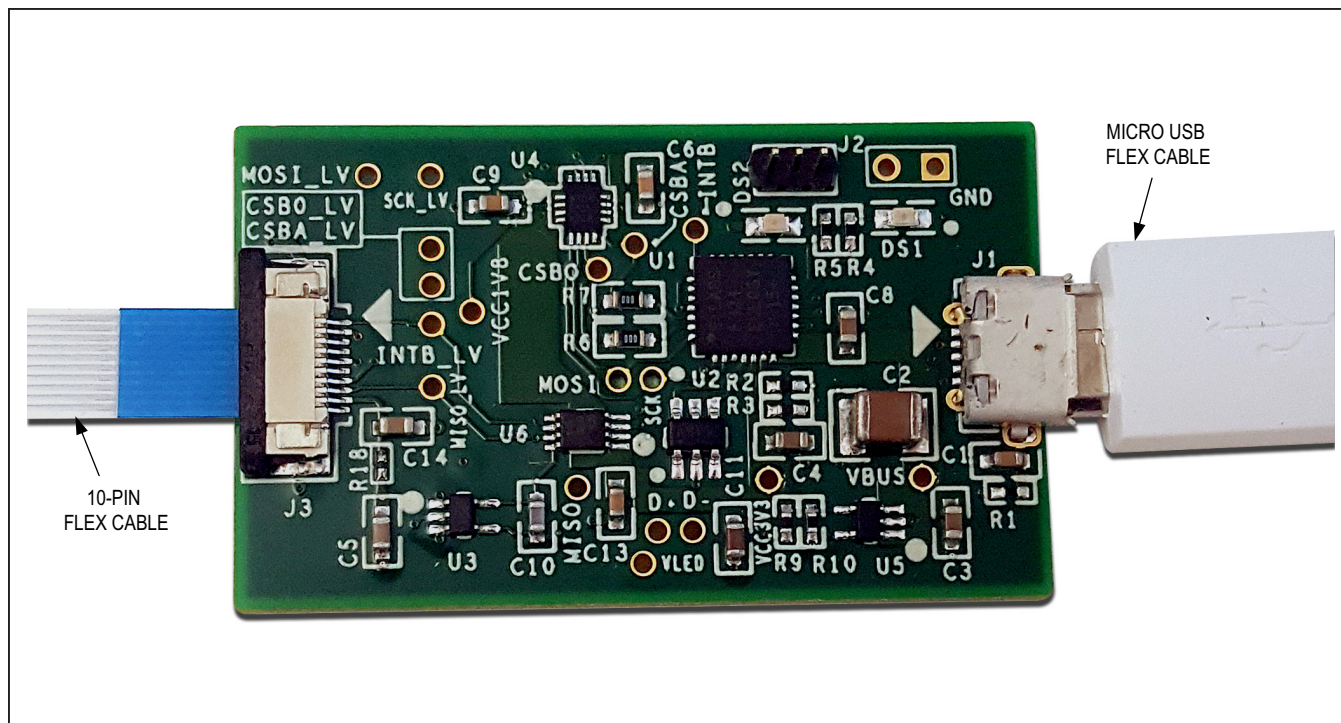
Figure 5. MAX30110 EV Kit—Hardware Setup (Micro-PCB)
