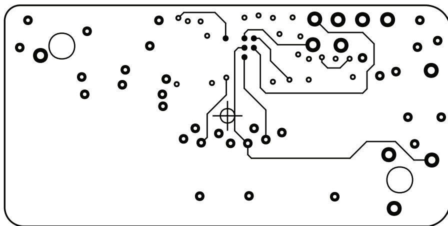
MAX30110 EV Kit—Level 5 SIGS
