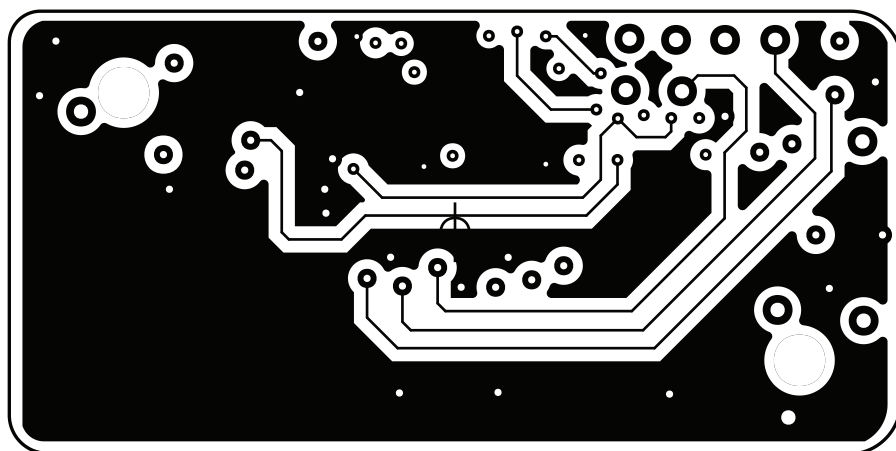
MAX30110 EV Kit—Level 2 SIGS
