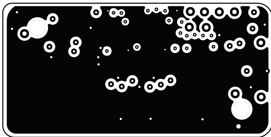
MAX30110 EV Kit—Level 3 GND
