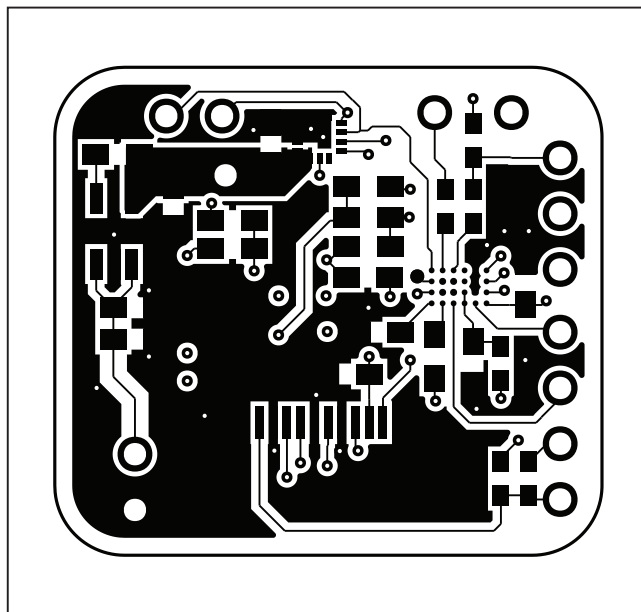
MAX30110 EV Kit—Bottom
