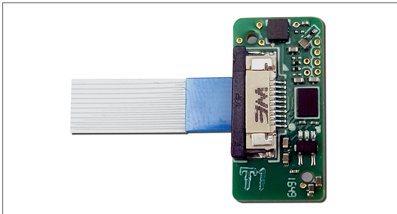
Figure 6. MAX30110 EV Kit—Hardware Setup (Sensor PCB 1)
