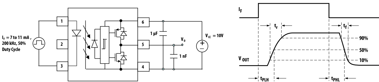
Figure 14: t r and t f Test Circuit and Waveforms
