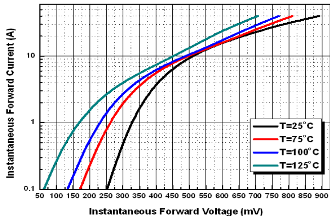
Figure 1. Typical Forward Characteristics per Diode
