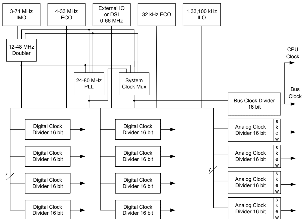
Figure 6-1. Clocking Subsystem
