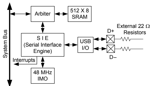
Figure 7-20. USB
