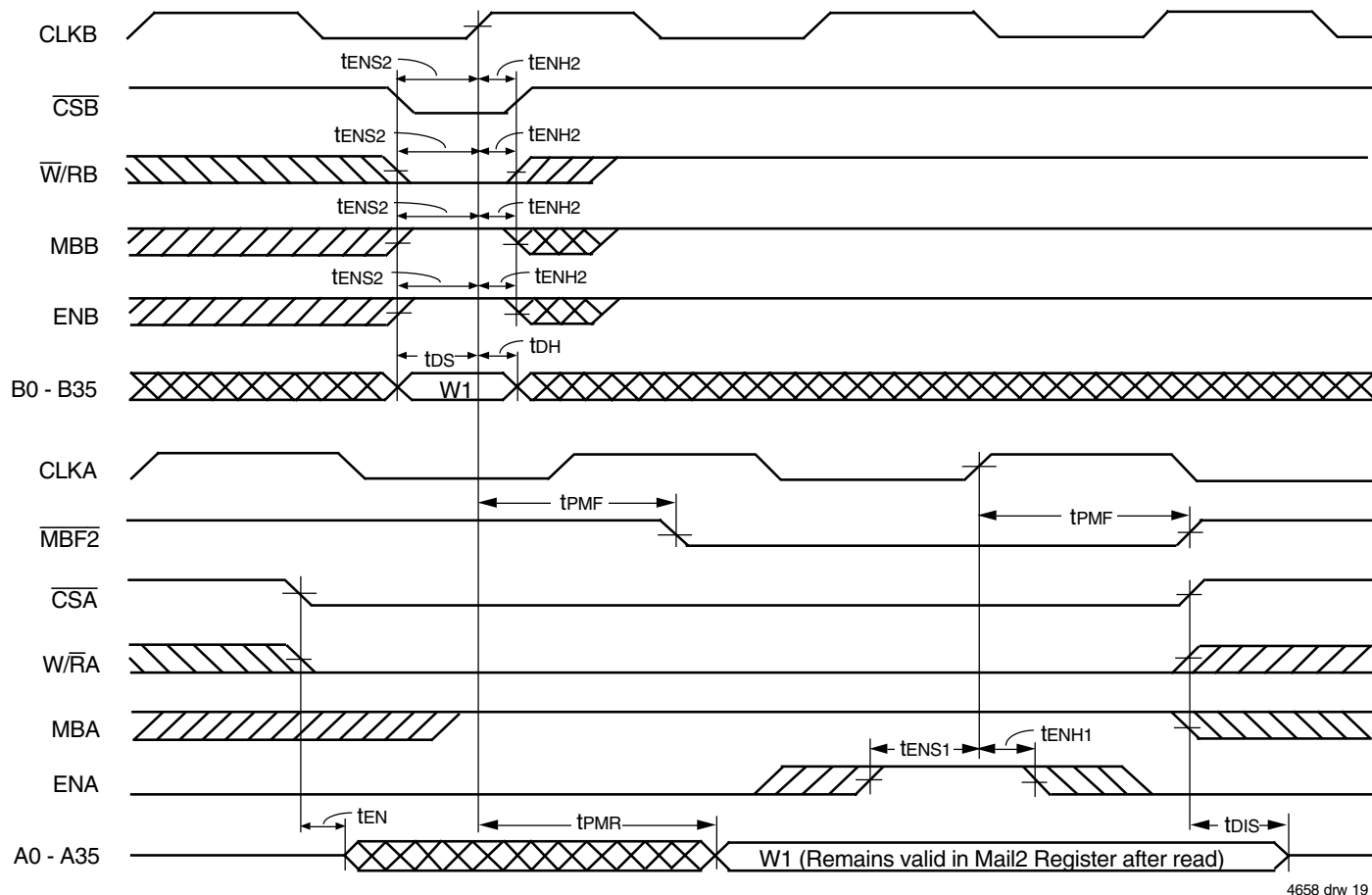
Figure 16. Timing for \overline{\text{Mail2}} Register and \overline{\text{MBF2}} Flag
