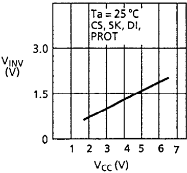
1.26 Input voltage V_{IN} ( V_{IL} , V_{IH} ) – Power supply voltage V_{CC}
