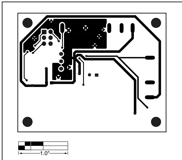
Figure 4. MAX5003 EV Kit PC Board Layout—Solder Side
