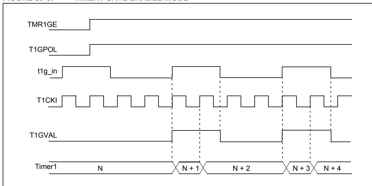
FIGURE 20-3: TIMER1 GATE ENABLE MODE
