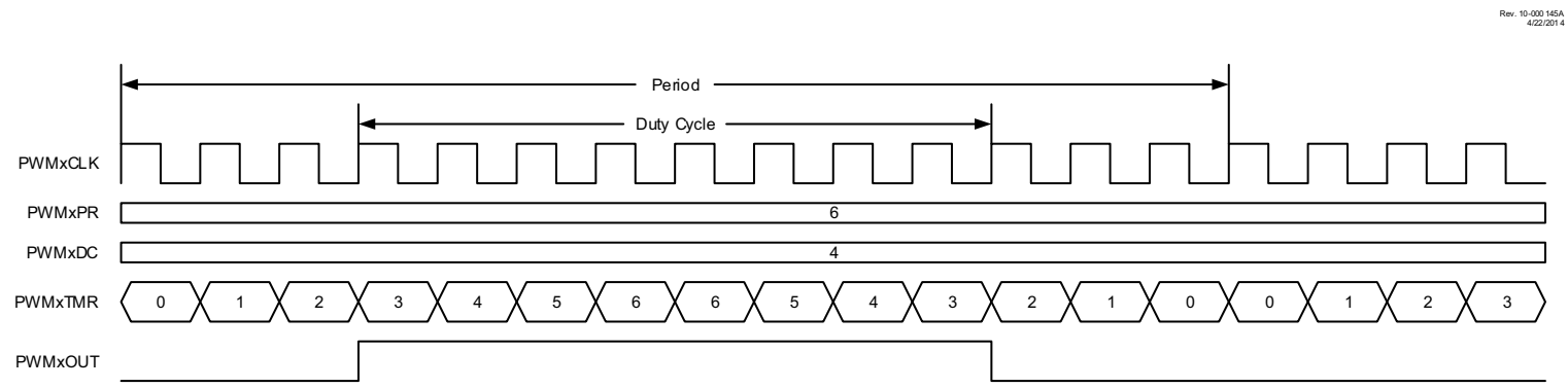
FIGURE 23-7: CENTER-ALIGNED PWM MODE TIMING DIAGRAM
