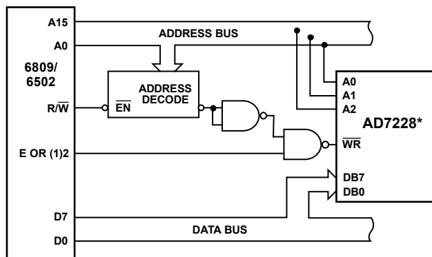
Figure 20. AD7228 to 6809/6502 Interface
