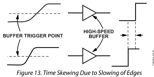
Figure 13. Time Skewing Due to Slowing of Edges
