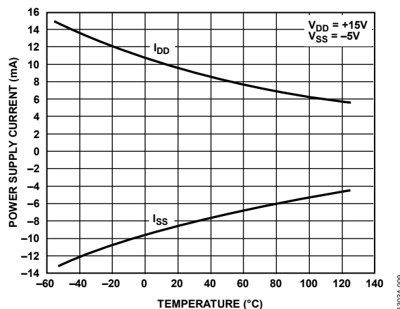
Figure 9. Power Supply Current vs. Temperature
