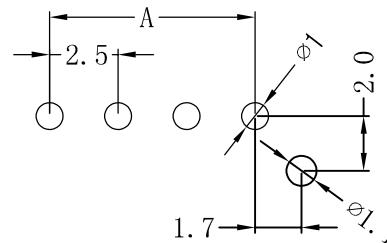
Recommand PCB Layout
