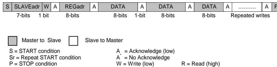
Figure 43: 2-WIRE Page Write
