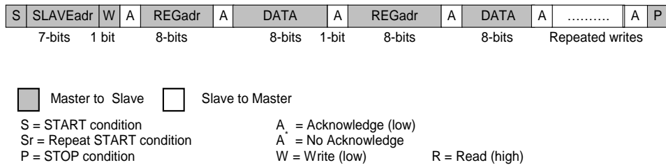
Figure 44: 2-WIRE Repeated Write
