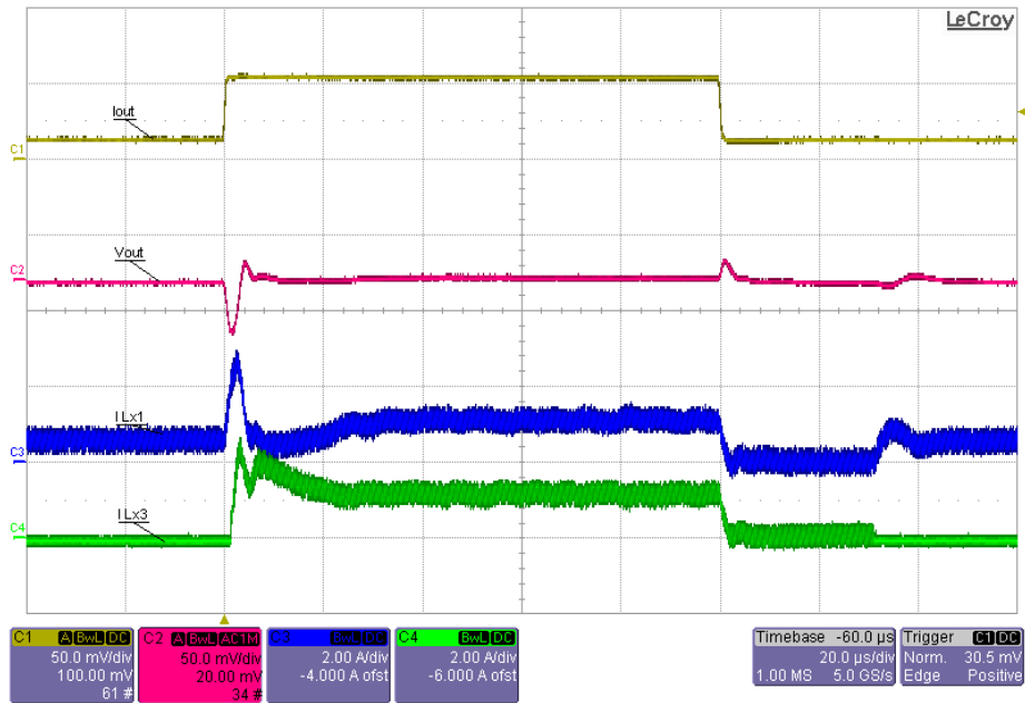
Figure 25: Transient Load, Auto, Dual Mode, 8-phases 1 to 10 A in 12 A/ \mu s, V_{DD} = 3.7 V, V_{OUT} = 1.0 V
