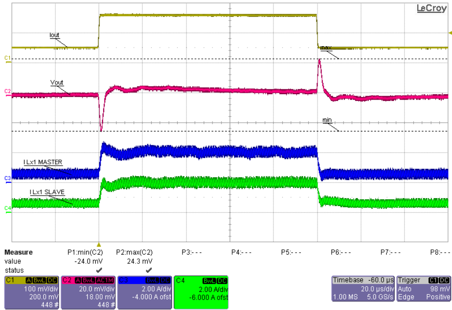
Figure 24: Transient Load, PWM, Dual Mode, 8-phases 5 to 17 A in 12 A/ \mu s, V_{DD} = 3.7 V, V_{OUT} = 1.0 V
