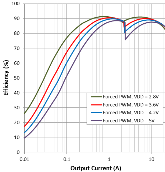
Figure 10: Efficiency vs Output Current V_{OUT} = 1.2\text{ V} , Dual Parallel Mode (24 A max)
