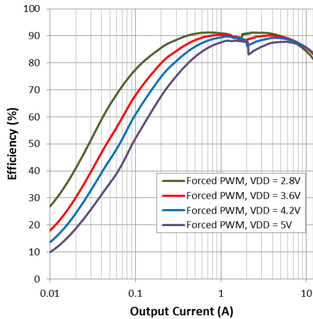
Figure 7: Efficiency vs Output Current V OUT = 1.2 V
