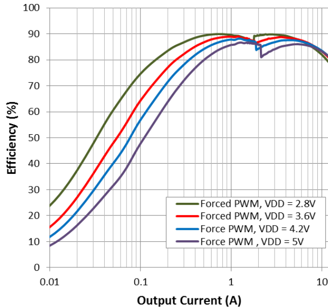
Figure 6: Efficiency vs Output Current V OUT = 1.0 V
