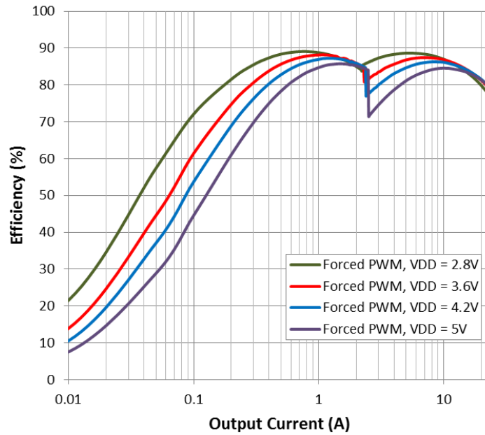
Figure 11: Efficiency vs Output Current V_{OUT} = 0.9\text{ V} , Dual Parallel Mode (24 A max)
