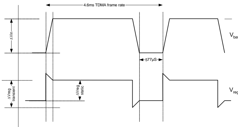
Figure 49: Line Regulation
