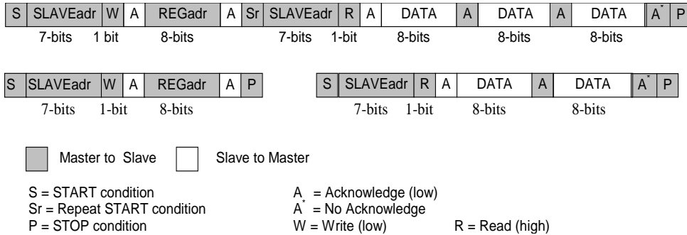
Figure 42: 2-WIRE Page Read
