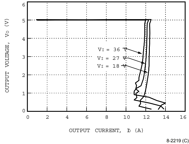
Figure 4. Typical JC050A Output Characteristics at Room Temperature
