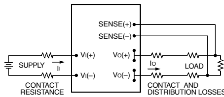
Figure 18. Effective Circuit Configuration for Single-Module Remote-Sense Operation
