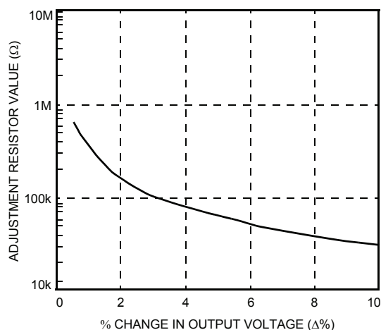
Figure 22. Resistor Selection for Increased Output Voltage
