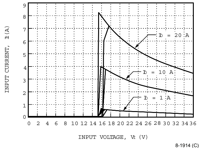
Figure 3. Typical JC100A Input Characteristics at Room Temperature
