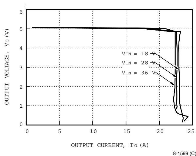
Figure 6. Typical JC100A Output Characteristics at Room Temperature.
