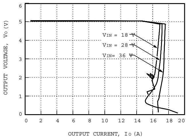
Figure 5. Typical JC075A Output Characteristics at Room Temperature.
