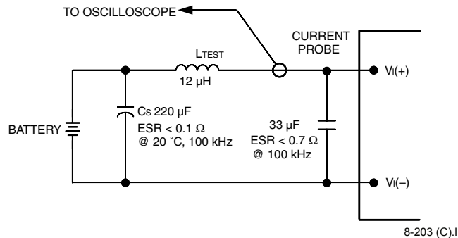
Figure 16. Output Voltage and Efficiency Measurement Test Setup
