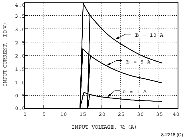
Figure 1. Typical JC050A Input Characteristics at Room Temperature
