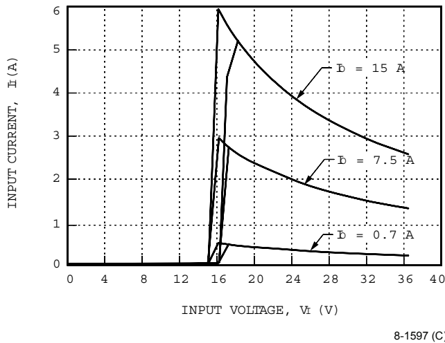
Figure 2. Typical JC075A Input Characteristics at Room Temperature
