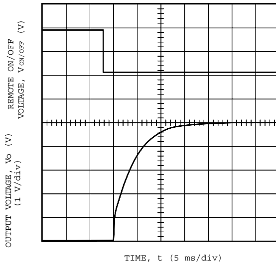
Figure 13. Typical Start-Up from Remote On/Off JC100A1; Io = Full Load
