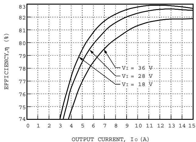
Figure 8. Typical JC075A Converter Efficiency vs. Output Current at Room Temperature
