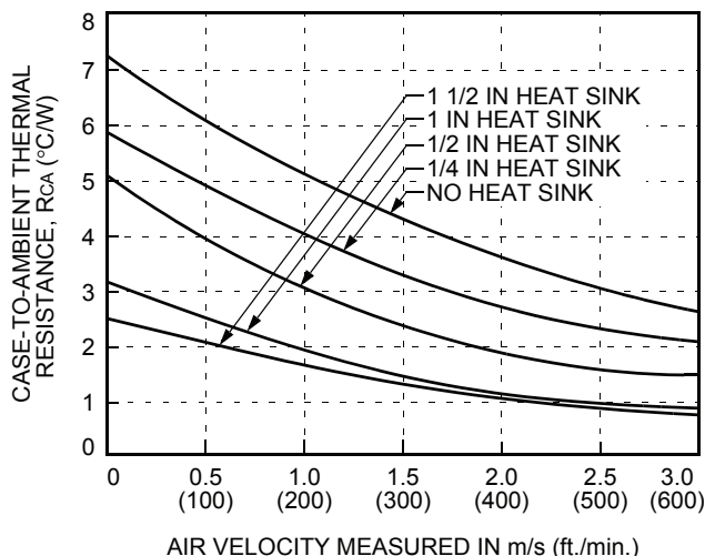
Figure 28. Case-to-Ambient Thermal Resistance Curves; Either Orientation
