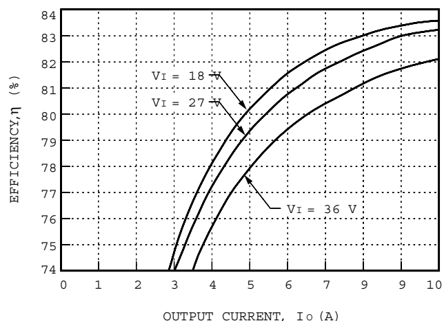
Figure 7. Typical JC050A Converter Efficiency vs. Output Current at Room Temperature
