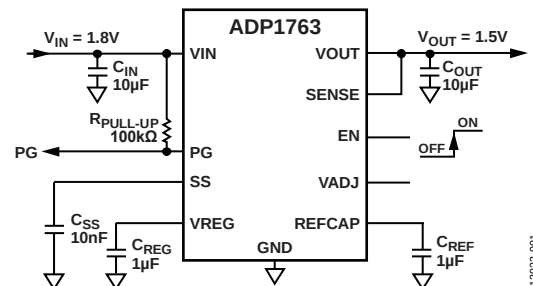
Figure 1. Fixed Output Operation
