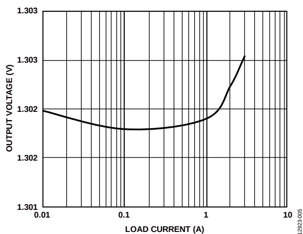
Figure 5. Output Voltage ( V_{OUT} ) vs. Load Current
