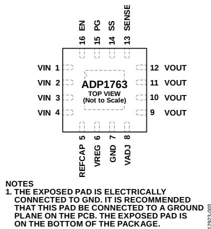
Figure 3. Pin Configuration
