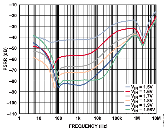
Figure 20. Power Supply Rejection Ratio (PSRR) vs. Frequency for Various Input Voltages, V_{OUT} = 1.3 V, Load Current = 3 A
