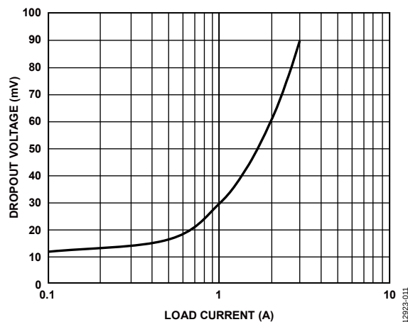
Figure 11. Dropout Voltage vs. Load Current, V_{OUT} = 1.3\text{ V}
