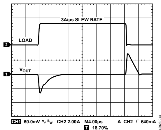
Figure 14. Load Transient Response, C_{OUT} = 10\text{ }\mu\text{F} , V_{IN} = 1.8\text{ V} , V_{OUT} = 1.3\text{ V}
