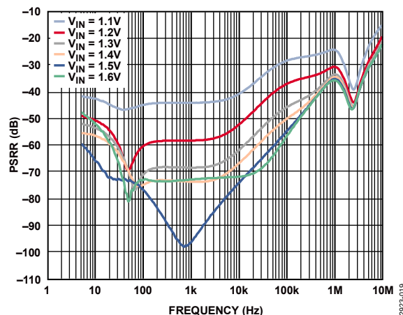
Figure 19. Power Supply Rejection Ratio (PSRR) vs. Frequency for Various Input Voltages, V_{OUT} = 0.9 V, Load Current = 3 A
