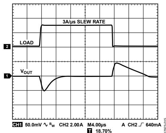
Figure 15. Load Transient Response, C_{OUT} = 47\text{ }\mu\text{F} , V_{IN} = 1.8\text{ V} , V_{OUT} = 1.3\text{ V}
