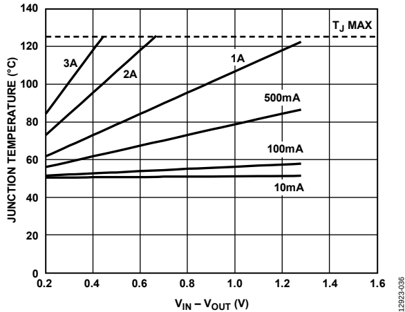
Figure 38. 6400 mm² of PCB Copper, T_A = 50^\circ\text{C}
