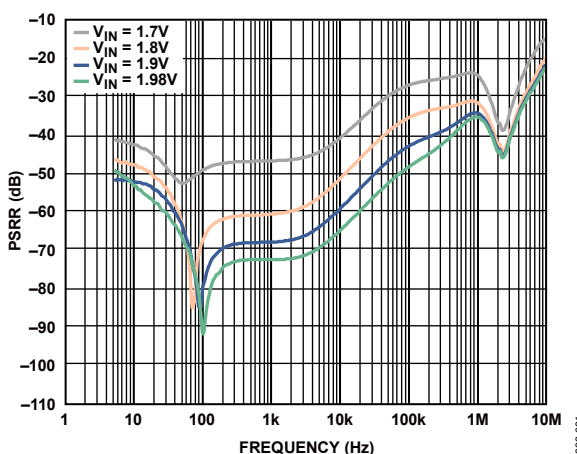
Figure 21. Power Supply Rejection Ratio (PSRR) vs. Frequency for Various Input Voltages, V_{OUT} = 1.5 V, Load Current = 3 A
