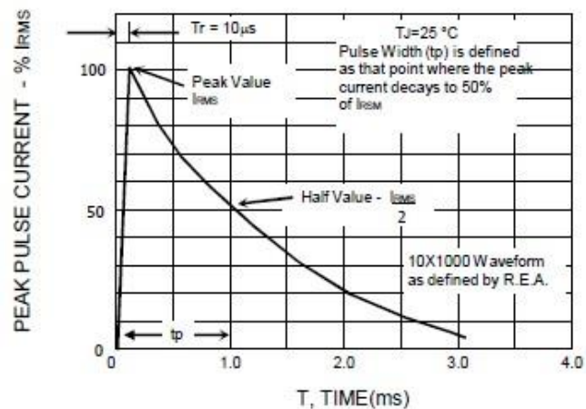
FIG.5 - PULSE WAVEFORM
