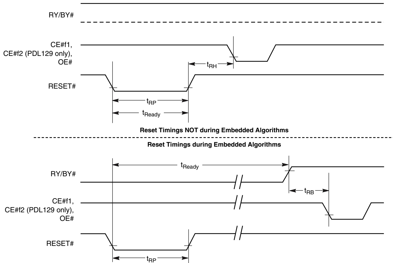
Figure 16. Reset Timings
