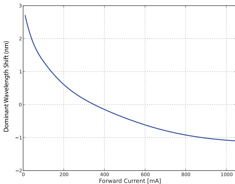
Figure 6b. Dominant wavelength shift vs. forward current for L0F2-Bxxx100005501 at T_j=25^{\circ}\text{C} .
