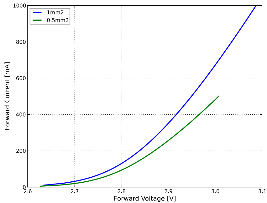
Figure 4. Typical forward current vs. forward voltage for L0F2-Bxxxxxxx0xxx1 at T_j=25^{\circ}\text{C} .
