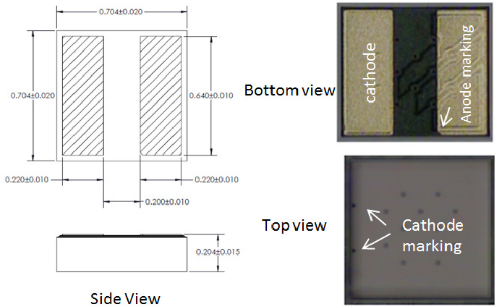
Figure 9a. Mechanical dimensions for LUXEON FlipChip Royal Blue L0F2-Bxxx050002751.
