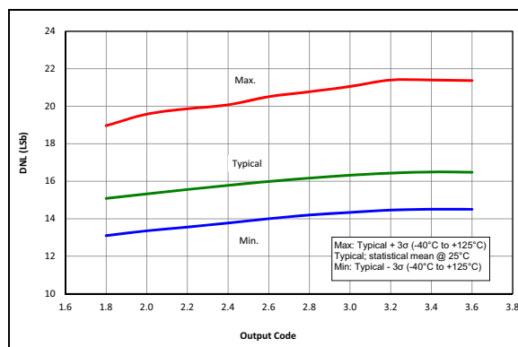
FIGURE 40-69: DAC DNL Error, VDD = 3.0V, PIC16LF19155/56/75/76/85/86 Only.
