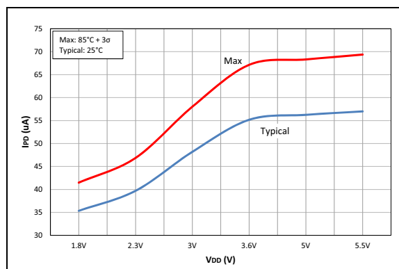
FIGURE 40-10: I_{PD} , Fixed Voltage Reference (FVR), PIC16F19155/56/75/76/85/86 Only.
