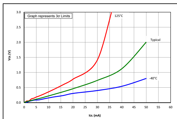
FIGURE 40-46: V_{OL} vs. I_{OL} Over Temperature, V_{DD} = 3.0V .
