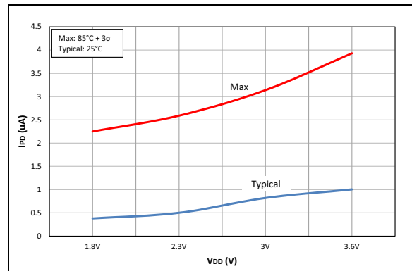
FIGURE 40-29: IPD, Secondary Oscillator (SOSC), PIC16LF19155/56/75/76/85/86 Only.
