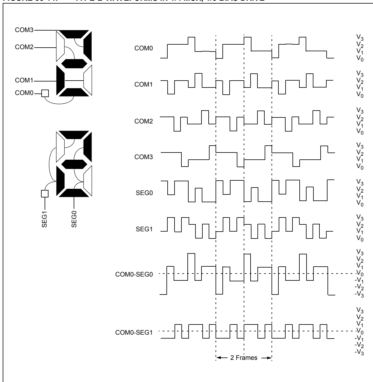
FIGURE 35-14: TYPE-B WAVEFORMS IN 1/4 MUX, 1/3 BIAS DRIVE
