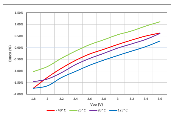
FIGURE 40-34: LFINTOSC Typical Frequency Error, PIC16LF19155/56/75/76/85/86 Only.
