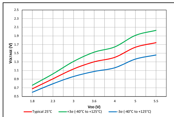
FIGURE 40-95: Schmitt Trigger Low Values.
