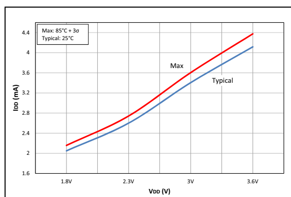
FIGURE 40-6: I_{DD} , HFINTOSC = 32 MHz with PLL, PIC16LF19155/56/75/76/85/86 Only.
