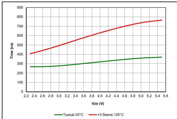
FIGURE 40-87: Comparator Response Time Rising Edge, PIC16F19155/56/75/76/85/86 Only.
