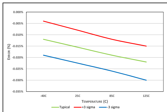
FIGURE 40-40: Low-Power Optimized HFINTOSC Frequency Error, VDD = 3V.
