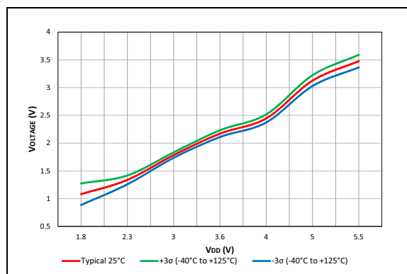
FIGURE 40-94: Schmitt Trigger High Values.
