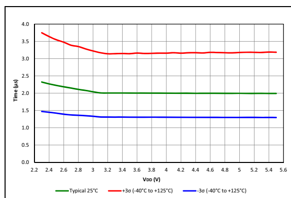
FIGURE 40-64: ADC RC Oscillator Period, PIC16F19155/56/75/76/85/86 Only.
