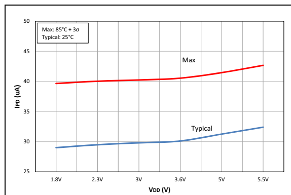
FIGURE 40-11: I_{PD} , Comparator C1, PIC16F19155/56/75/76/85/86 Only.
