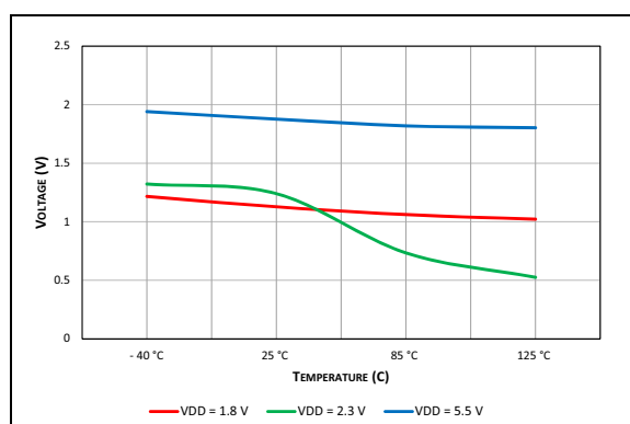
FIGURE 40-100: Typical Input High Voltage with SMBus Level.
