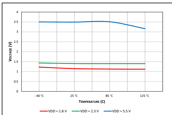
FIGURE 40-98: Typical Input High Voltage with I²C Level.
