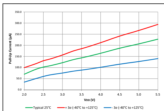
FIGURE 40-41: Weak Pull-Up Current, PIC16F19155/56/75/76/85/86 Only.
