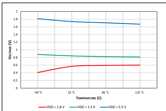
FIGURE 40-97: Typical Input Low Voltage with I²C Level.
