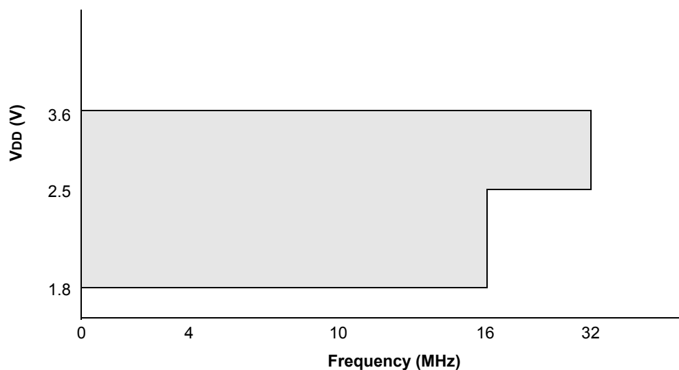
FIGURE 39-2: VOLTAGE FREQUENCY GRAPH, -40^{\circ}\text{C} \leq T_A \leq +125^{\circ}\text{C} , PIC16(L)F19155/56/75/76/85/86 ONLY
