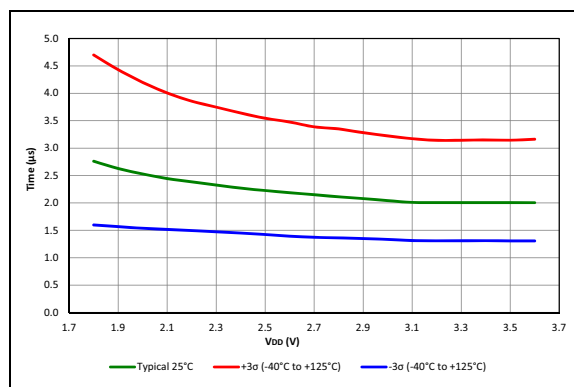
FIGURE 40-63: ADC RC Oscillator Period, PIC16LF19155/56/75/76/85/86 Only.
