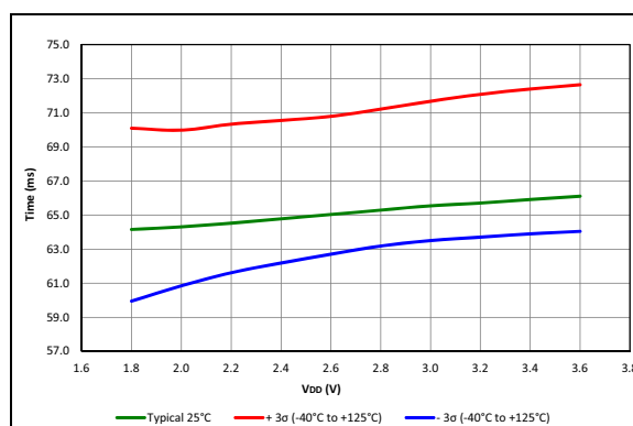
FIGURE 40-107: PWRT Period, PIC16LF19155/56/75/76/85/86 Only.
