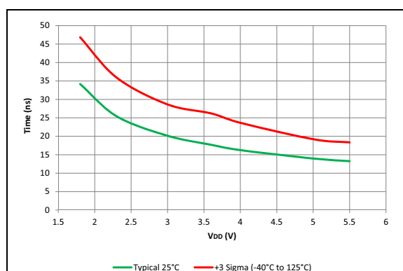
FIGURE 40-101: Rise Time, Slew Rate Control Enabled.
