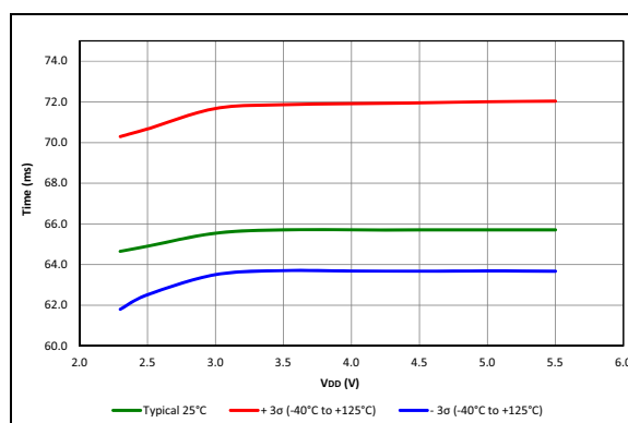
FIGURE 40-106: PWRT Period, PIC16F19155/56/75/76/85/86 Only.
