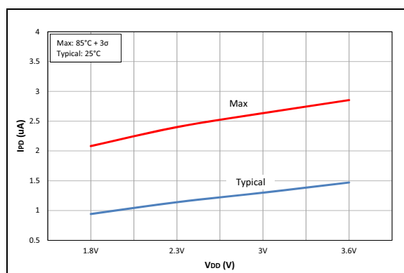
FIGURE 40-23: IPD, LP Comparator C2, PIC16LF19155/56/75/76/85/86 Only.
