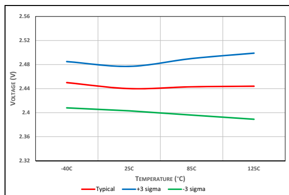
FIGURE 40-53: LPBOR Reset Voltage.
