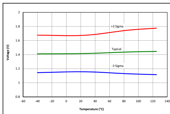
FIGURE 40-105: POR Rearm Voltage.
