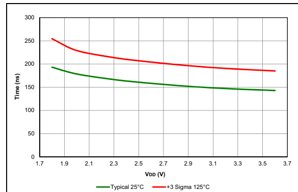
FIGURE 40-84: Comparator Response Time Falling Edge, PIC16LF19155/56/75/76/85/86 Only.
