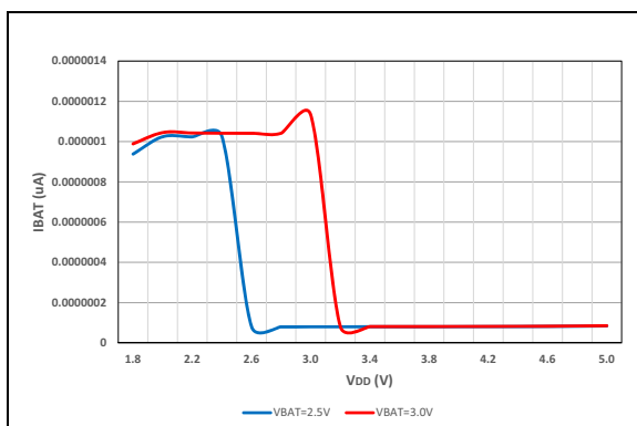
FIGURE 40-32: Typical IBAT.
