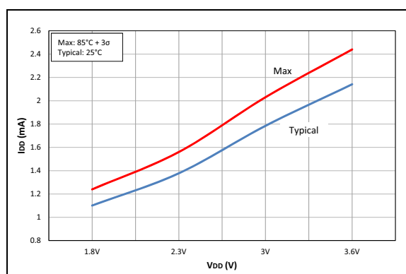
FIGURE 40-5: I_{DD} , HFINTOSC = 16 MHz, PIC16LF19155/56/75/76/85/86 Only.
