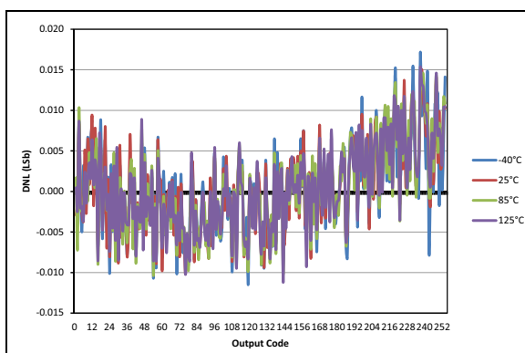
FIGURE 40-67: Typical DAC DNL Error, VDD = 5.0V, VREF = External 5.0V PIC16F19155/56/75/76/85/86 Only.
