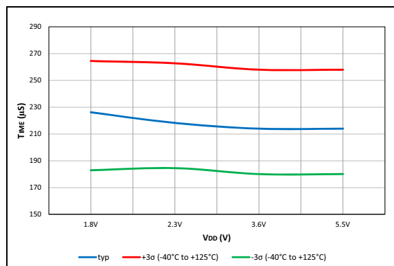
FIGURE 40-112: LFINTOSC Wake-up from Sleep Start-up Time
