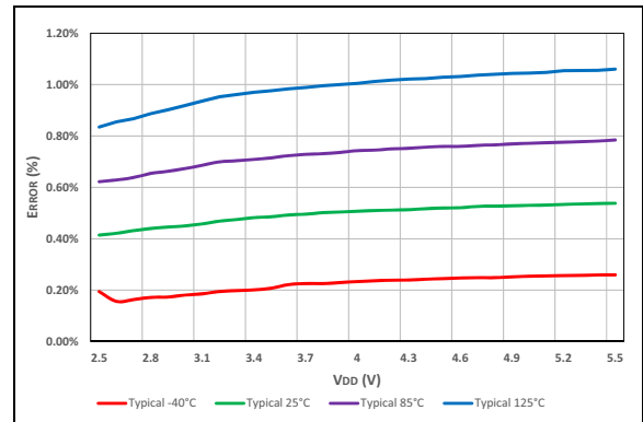
FIGURE 40-90: Typical FVR Voltage 1x Error, PIC16F19155/56/75/76/85/86 Only.
