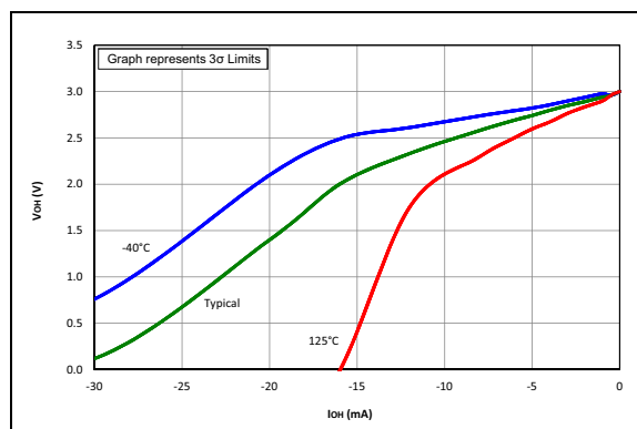
FIGURE 40-45: V_{OH} vs. I_{OH} Over Temperature, V_{DD} = 3.0V .
