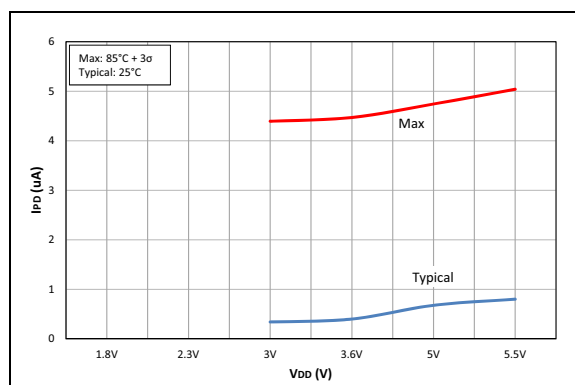
FIGURE 40-16: IPD, Low-Power Brown-Out Reset (LPBOR), PIC16F19155/56/75/76/85/86 Only.
