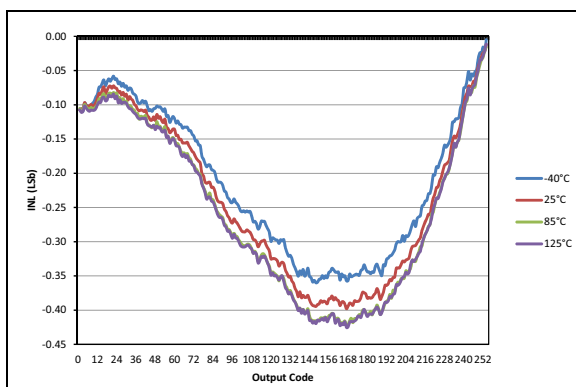
FIGURE 40-66: Typical DAC INL Error, VDD = 3.0V, VREF = External 3.0V.
