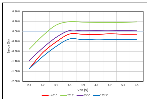
FIGURE 40-33: LFINTOSC Typical Frequency Error, PIC16LF19155/56/75/76/85/86 Only.
