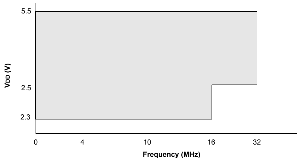
FIGURE 39-1: VOLTAGE FREQUENCY GRAPH, -40^{\circ}\text{C} \leq T_A \leq +125^{\circ}\text{C} , PIC16F19155/56/75/76/85/86 ONLY
