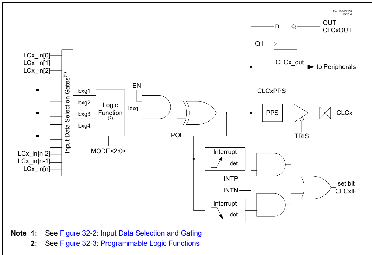
FIGURE 32-1: CLCx SIMPLIFIED BLOCK DIAGRAM
