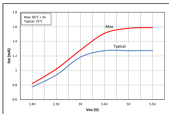
FIGURE 40-4: I_{DD} , Idle Mode, HFINTOSC = 16 MHz, PIC16F19155/56/75/76/85/86 Only.
