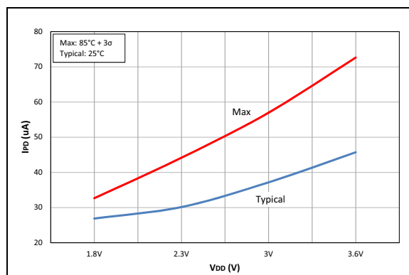
FIGURE 40-21: IPD, Fixed Voltage Reference (FVR), PIC16LF19155/56/75/76/85/86 Only.
