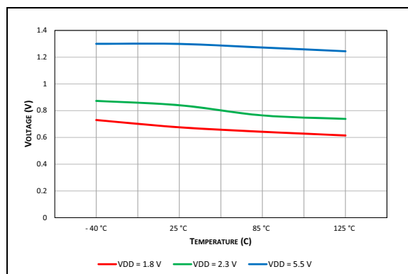
FIGURE 40-99: Typical Input Low Voltage with SMBus Level.
