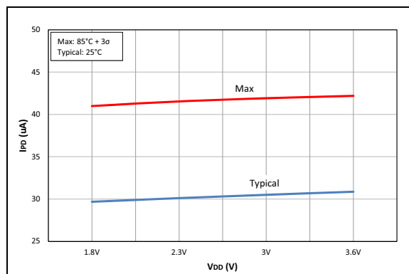
FIGURE 40-22: IPD, Comparator C1, PIC16LF19155/56/75/76/85/86 Only.
