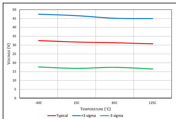
FIGURE 40-52: Brown-Out Reset Hysteresis, Trip Point (BORV = 1).
