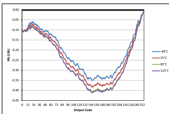
FIGURE 40-68: Typical DAC INL Error, VDD = 5.0V, VREF = External 5.0V PIC16F19155/56/75/76/85/86 Only
