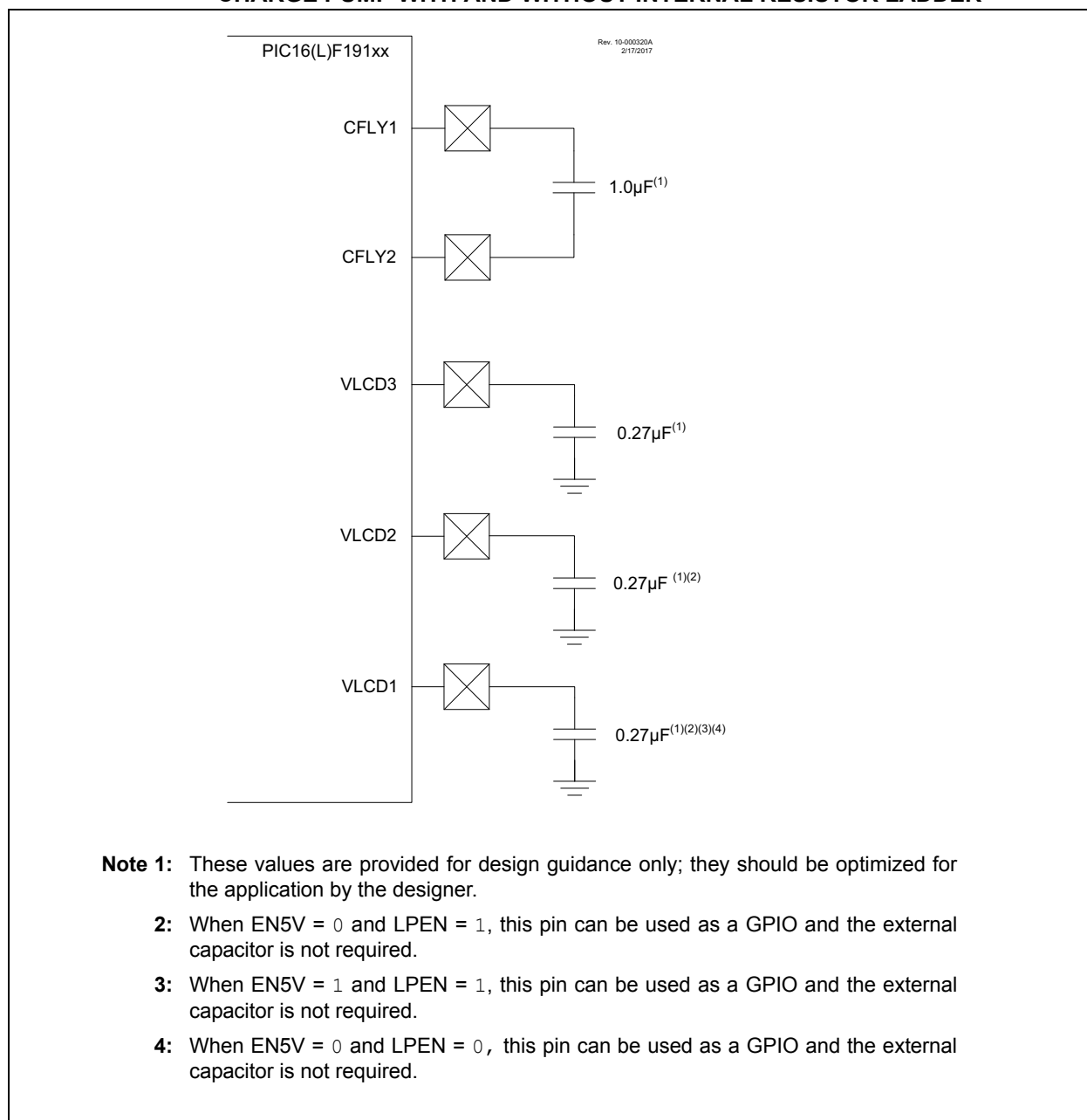
FIGURE 35-5: LCD REGULATOR CONNECTIONS FOR LCD VOLTAGE SUPPLIED FROM CHARGE PUMP WITH AND WITHOUT INTERNAL RESISTOR LADDER
