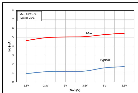
FIGURE 40-15: IPD, Low_frequency Oscillator/WDT, PIC16F19155/56/75/76/85/86 Only.
