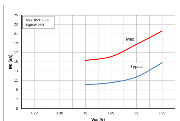
FIGURE 40-17: IPD, Brown-Out Reset (BOR), PIC16F19155/56/75/76/85/86 Only.
