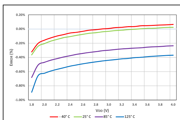
FIGURE 40-35: HFINTOSC Typical Frequency Error, PIC16LF19155/56/75/76/85/86 Only.
