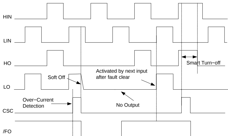
Figure 12. Inter-Lock Function
