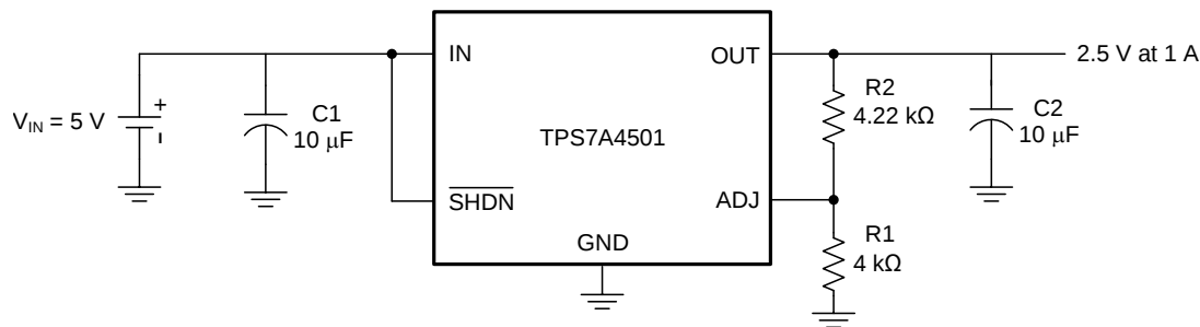
Figure 33. Adjustable Output Voltage Operation
