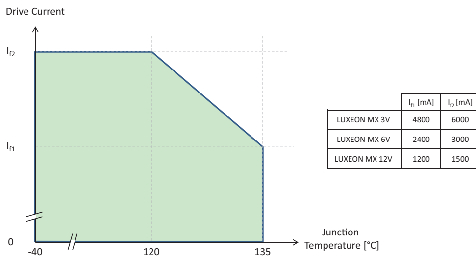
Figure 1. Maximum permissible operating conditions for LUXEON MX.
