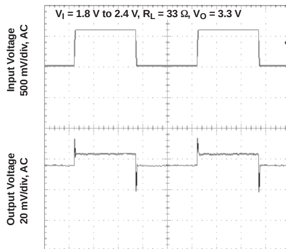
TPS61071 LINE TRANSIENT RESPONSE
