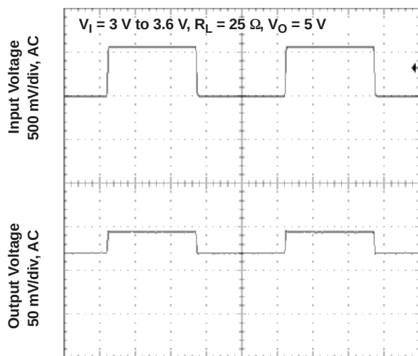
TPS61071 LINE TRANSIENT RESPONSE
