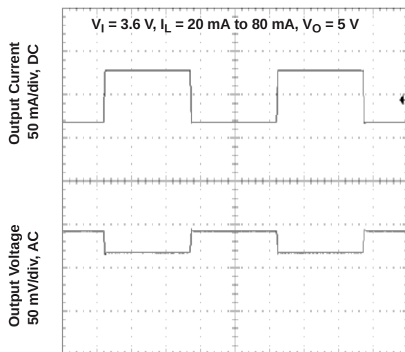
TPS61071 LOAD TRANSIENT RESPONSE
