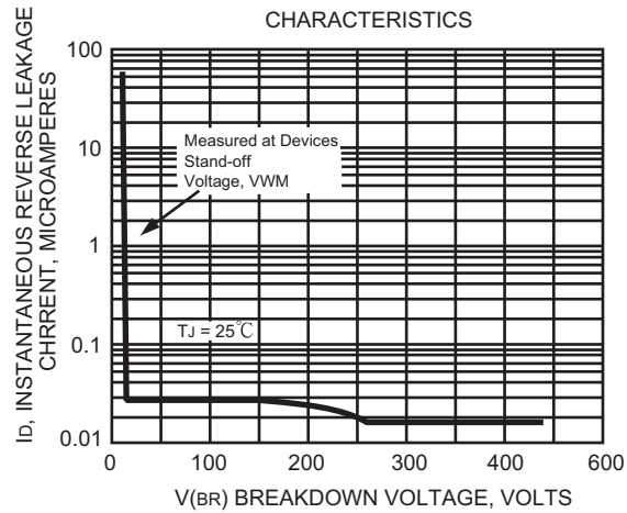
FIG. 7 - TYPICAL REVERSE LEAKAGE
