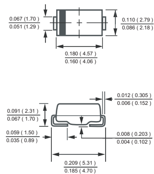
DO-214AC
