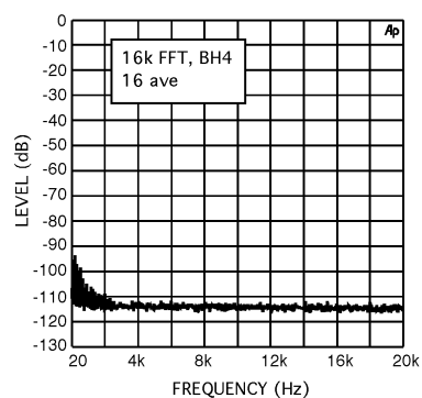
DAC Noise Floor
