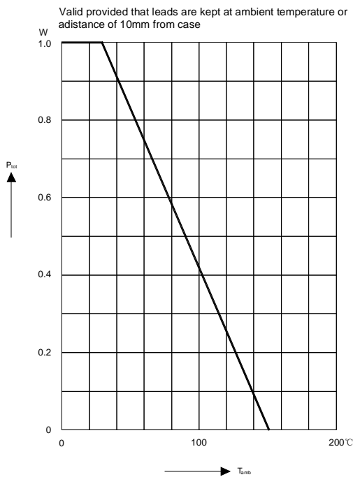
FIG.1-ADMISSIBLE POWER DISSIPATION VERSUS AMBIENT TEMPERATURE
