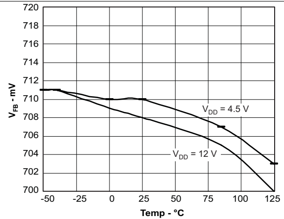
Figure 20. Reference Voltage vs Temperature
