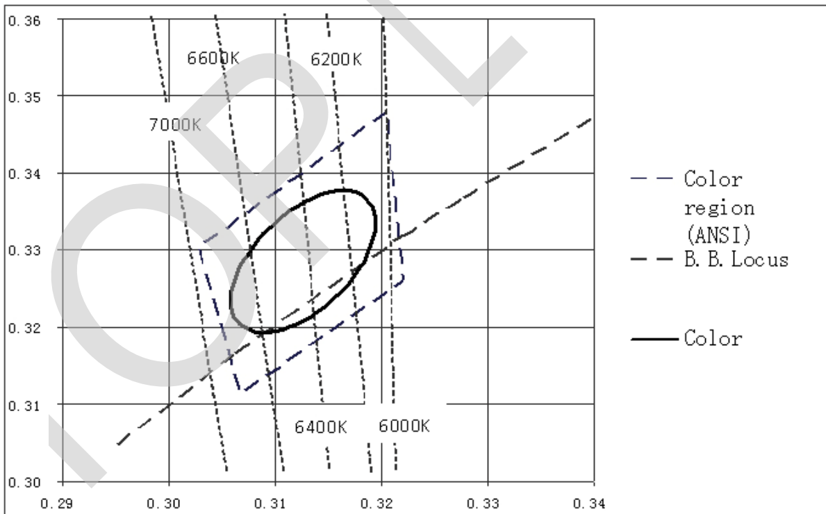
Chromaticity Diagram
