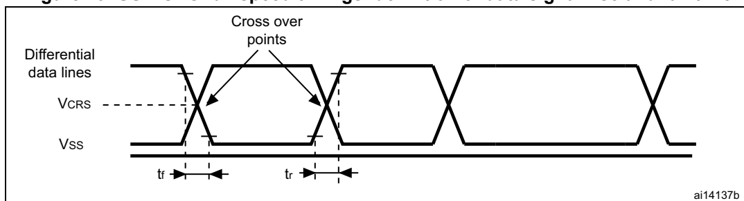
Figure 49. USB OTG full speed timings: definition of data signal rise and fall time
