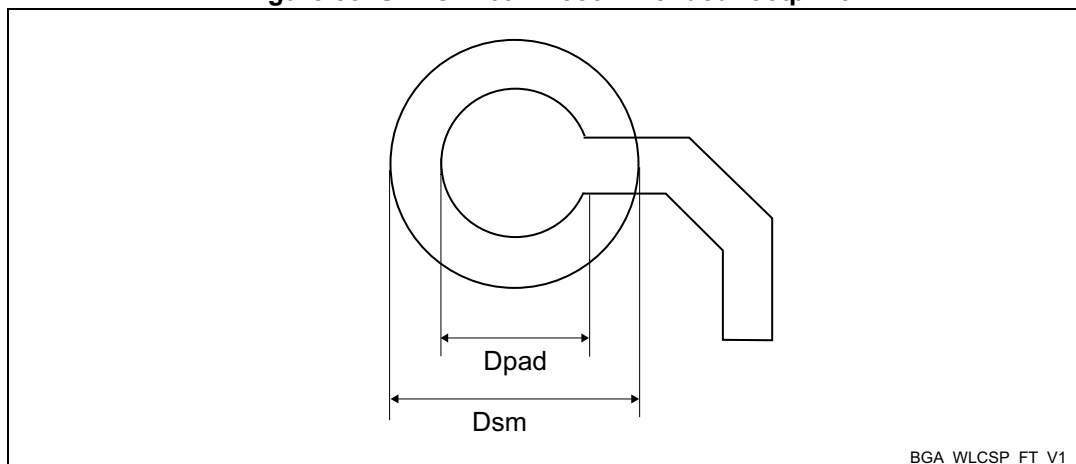
Figure 88. UFBGA169 - Recommended footprint
