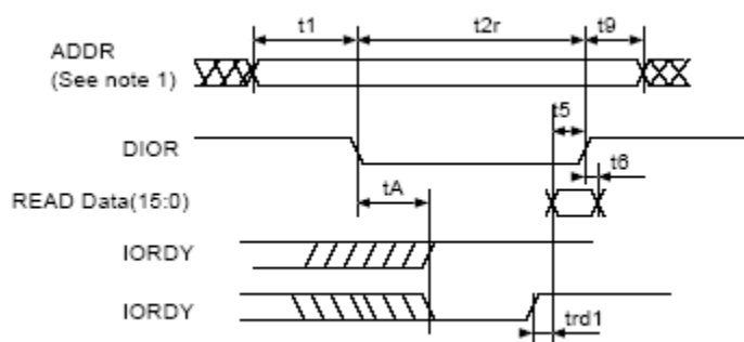
Figure 10. PIO Read Timing Diagram
