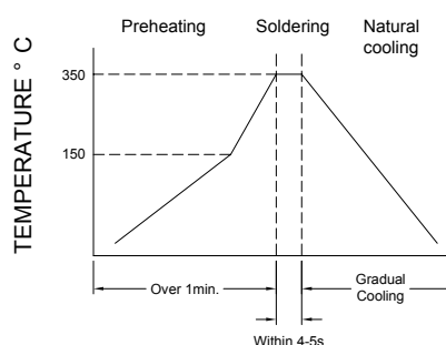
Figure 2. Iron Soldering
