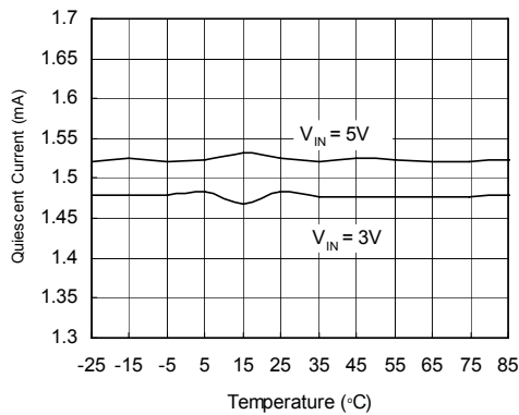
Quiescent Current vs. Temperature(G965-15)
