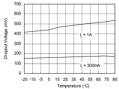
Dropout Voltage vs. Temperature(G965-15)
