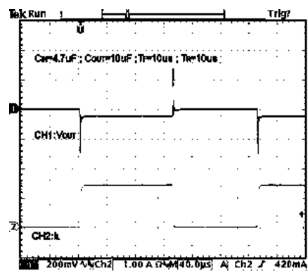
Load Transient Response(G965-18)
