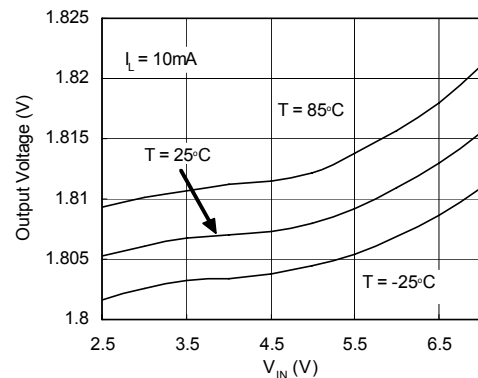
Output Voltage vs. V_{IN} (G965-18)
