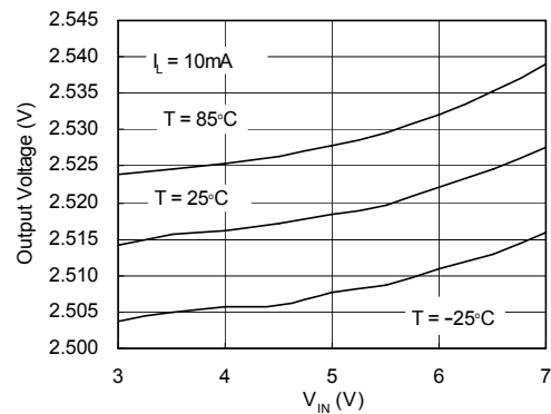
Output Voltage vs. V_{IN} (G965-25)
