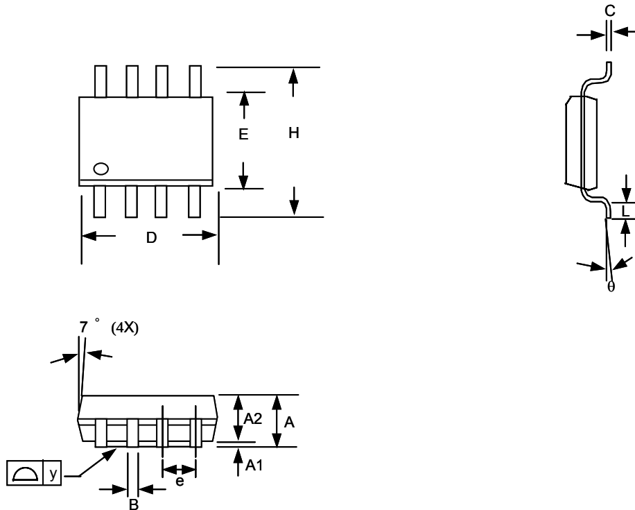
SOP-8 Package
