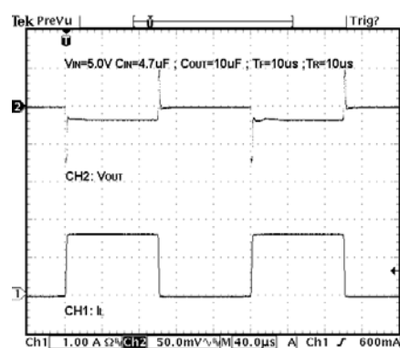
Load Transient Response(G965-25)
