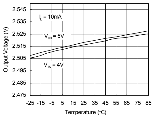
Output Voltage vs. Temperature(G965-25)
