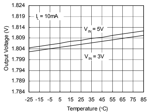
Output Voltage vs. Temperature(G965-18)
