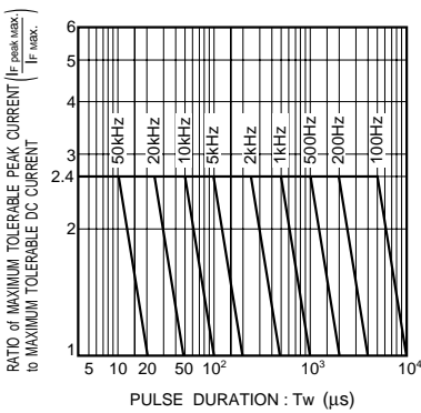
Fig. 20 Maximum tolerable peak current vs. pulse duration
