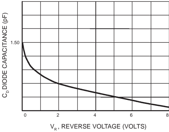
Figure 4. Capacitance
