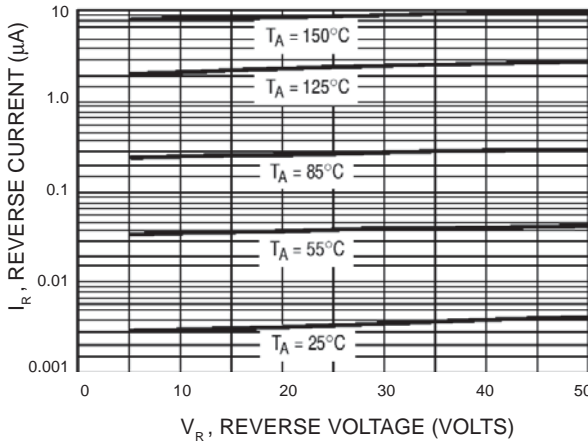
Figure 3. Leakage Current
