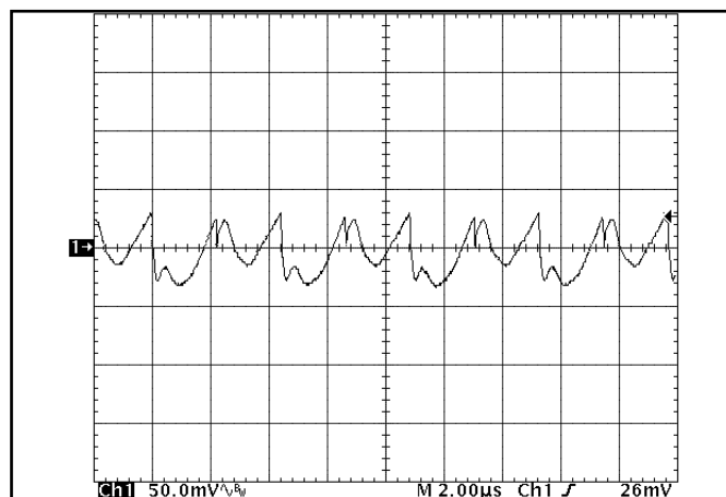
Figure 16: Output Voltage Ripple at nominal input voltage and rated load current (50 mV/div). Load capacitance: 1\ \mu F ceramic capacitor and 10\ \mu F tantalum capacitor. Bandwidth: 20 MHz. See Figure 13.
