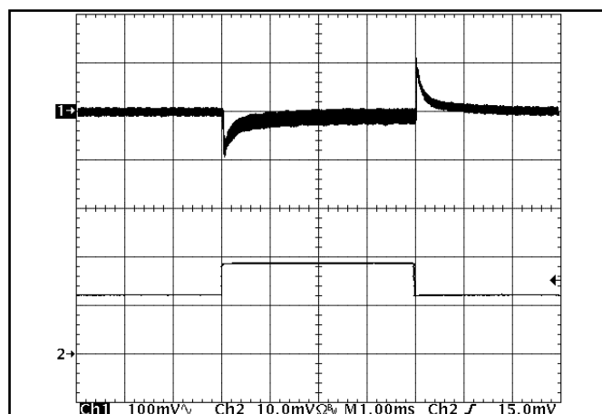
Figure 12: Output voltage response to step-change in load current (50%-75%-50% of I_{out(max)} ; dI/dt = 5\text{A}/\mu\text{s} ). Load cap: 470 \mu\text{F} , 30 m \Omega ESR tantalum cap and 1 \mu\text{F} ceramic cap. Ch 1: V_{out} (100mV/div), Ch 2: I_{out} (10A/div).
