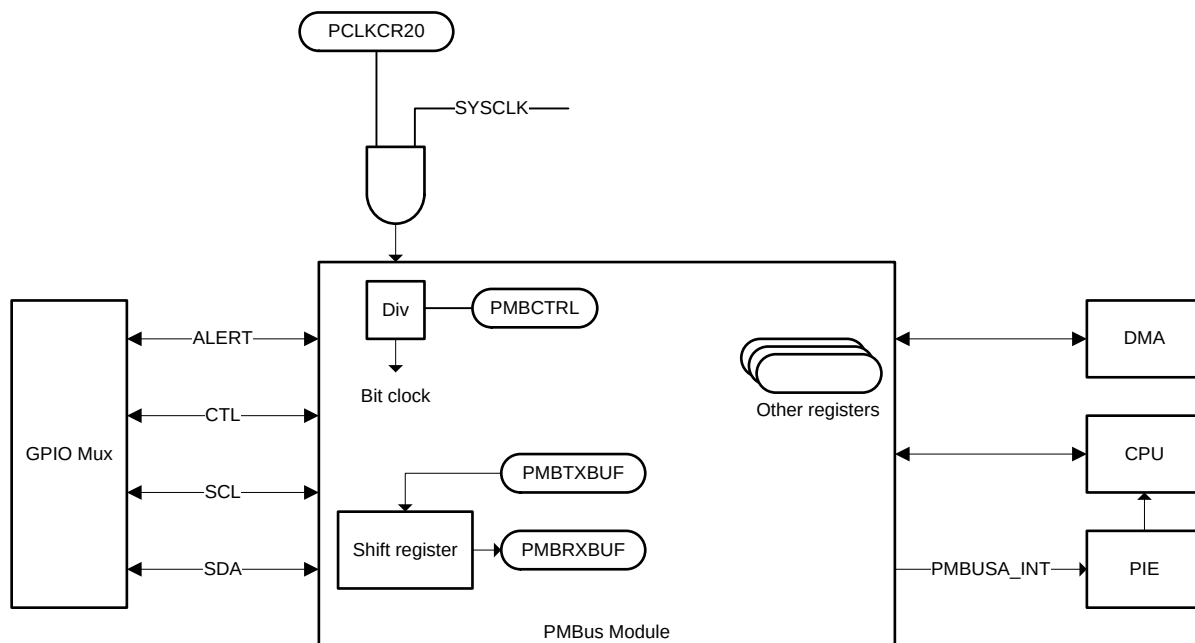
Figure 5-63. PMBus Block Diagram
