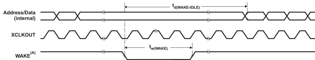
Figure 5-25. IDLE Entry and Exit Timing Diagram
