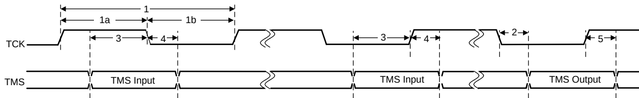
Figure 5-19. cJTAG Timing
