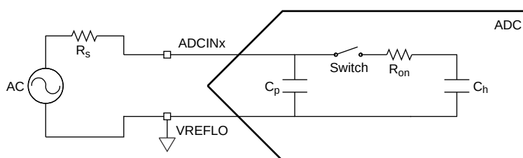
Figure 5-33. Input Model
