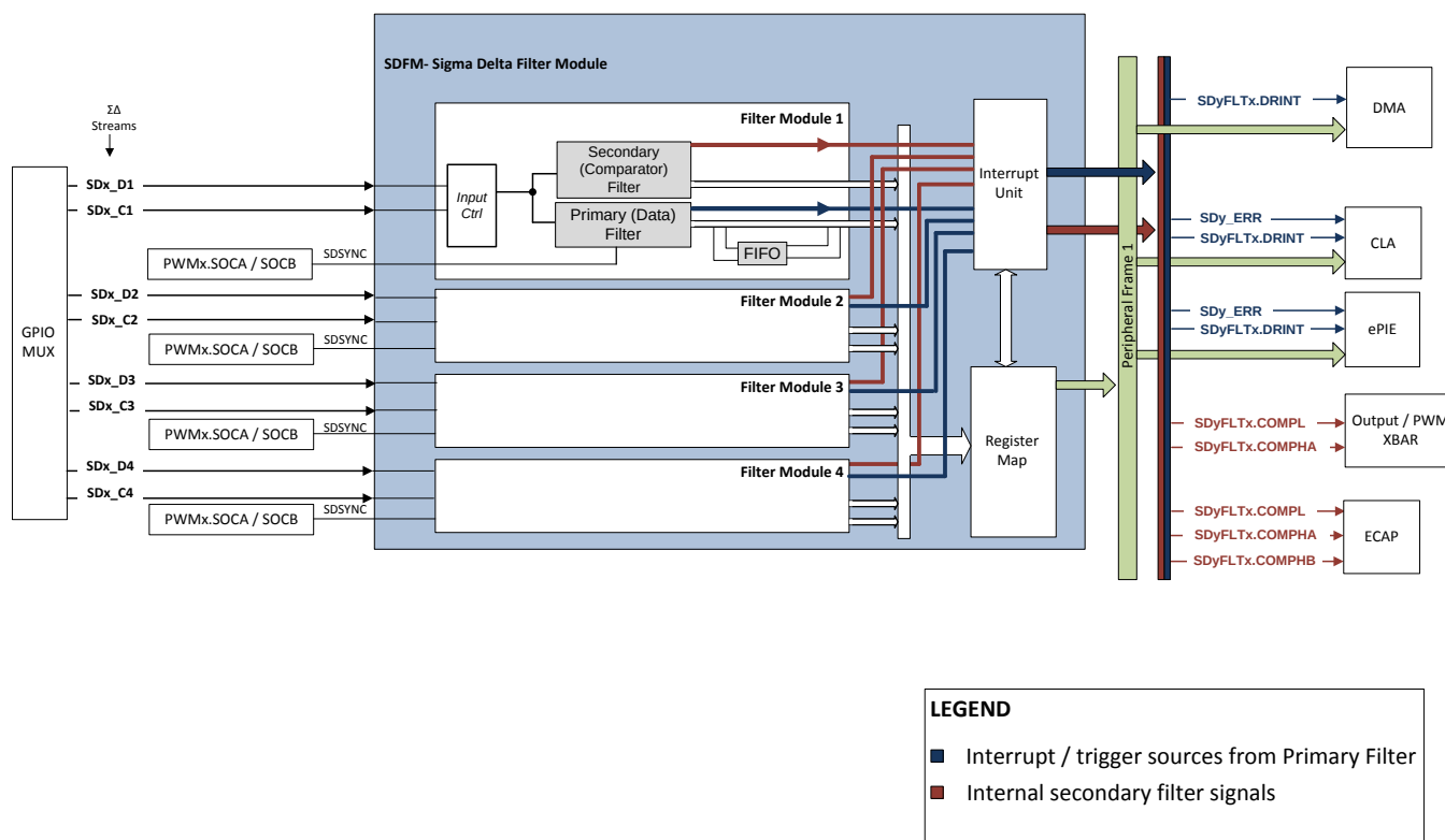
Figure 5-56. SDFM Block Diagram
