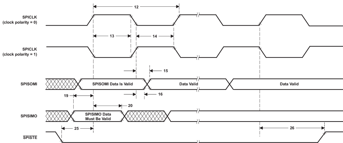
Figure 5-69. SPI Slave Mode External Timing (Clock Phase = 1)
