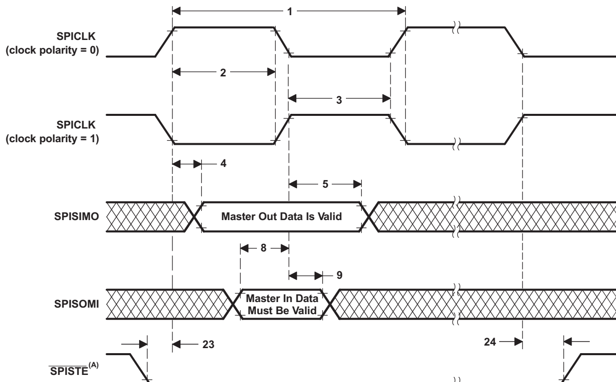
Figure 5-70. High-Speed SPI Master Mode External Timing (Clock Phase = 0)
