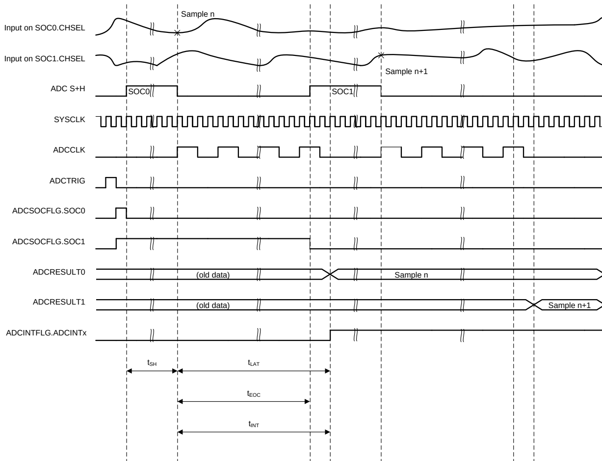
Figure 5-34. ADC Timings
