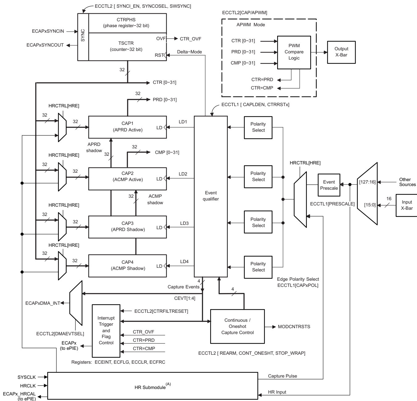
Figure 5-47. HRCAP Block Diagram
