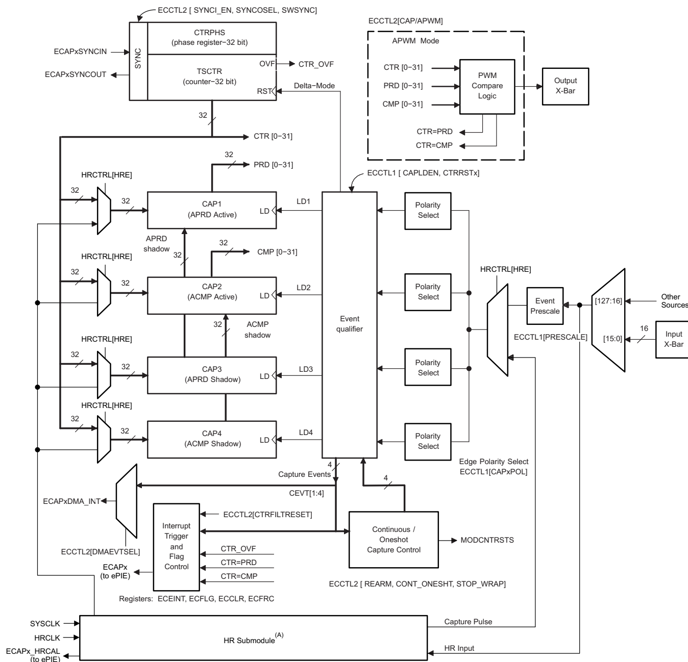
Figure 5-46. eCAP Block Diagram
