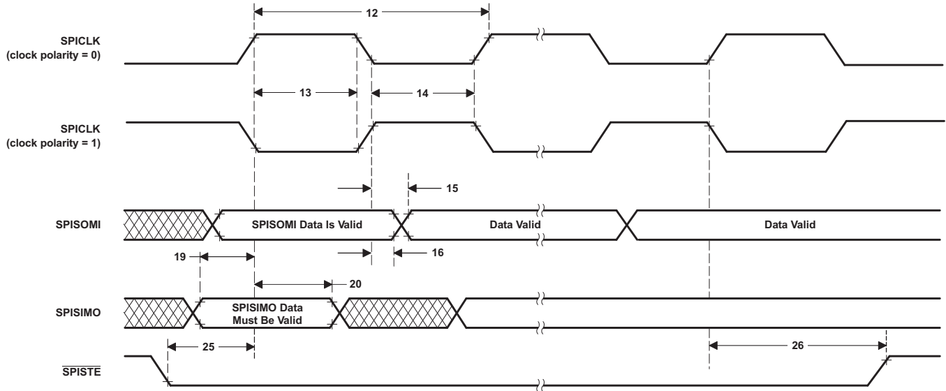
Figure 5-73. High-Speed SPI Slave Mode External Timing (Clock Phase = 1)
