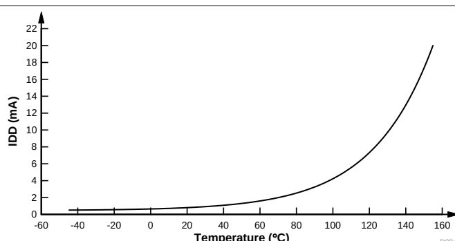
Figure 5-4. Halt Current Versus Temperature (°C)
