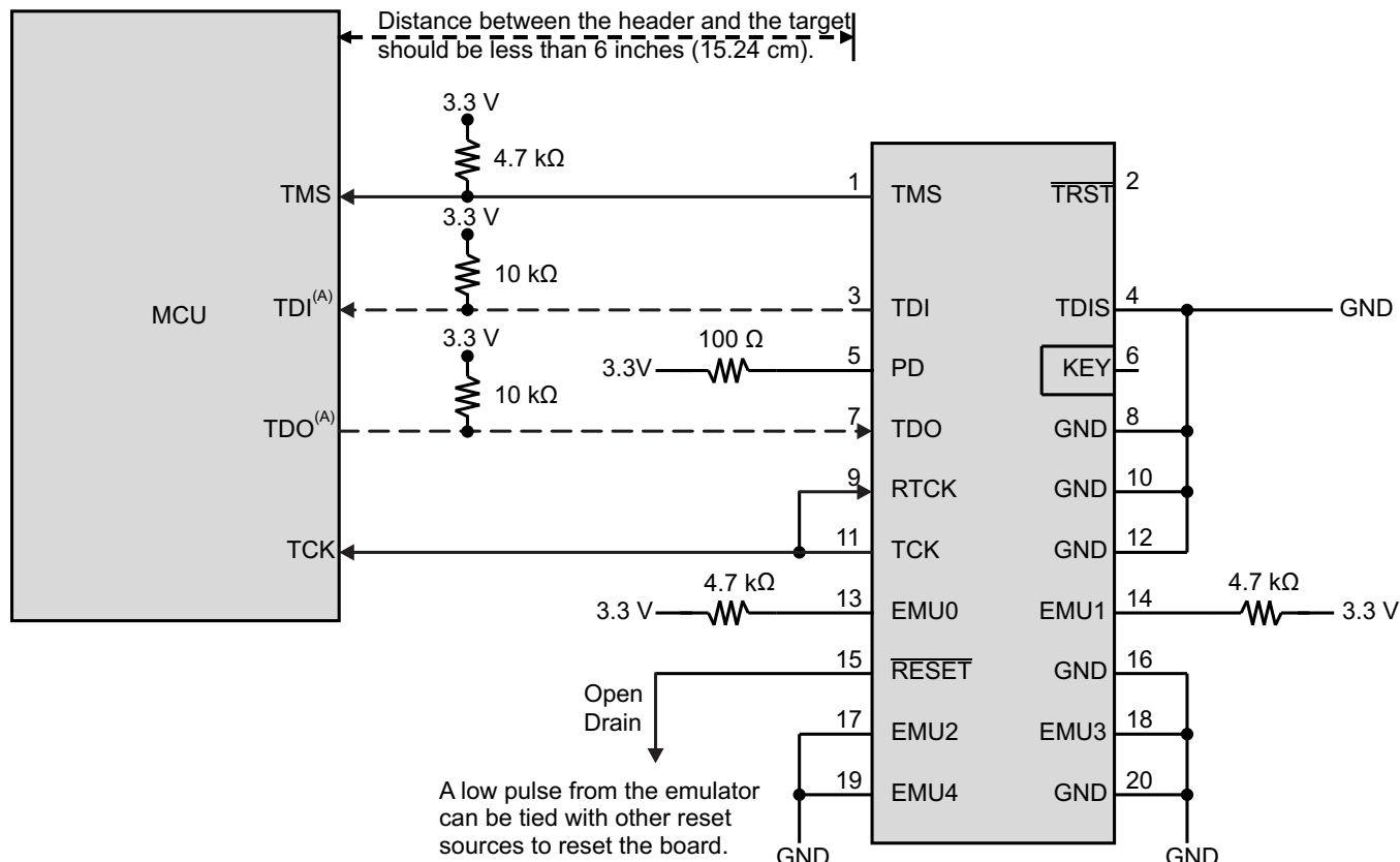
Figure 5-17. Connecting to the 20-Pin JTAG Header
