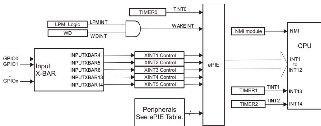
Figure 5-23. Device Interrupt Architecture
