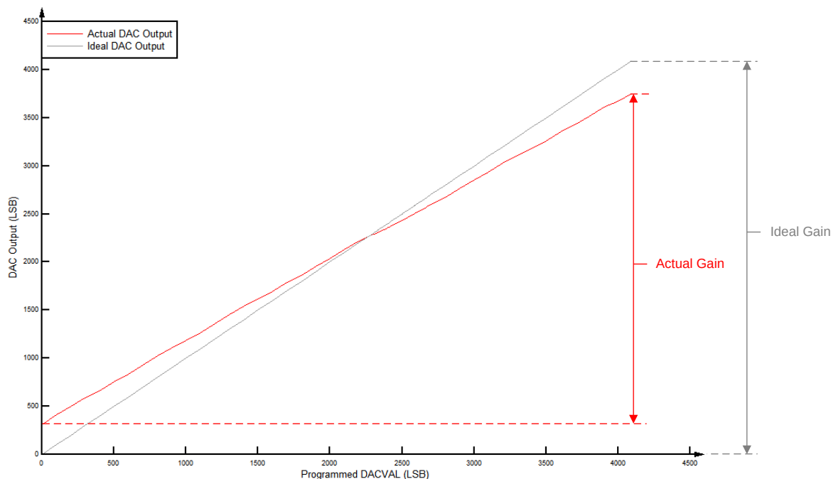
Figure 5-44. CMPSS DAC Static Gain
