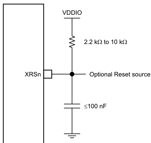
Figure 5-6. Reset Circuit
