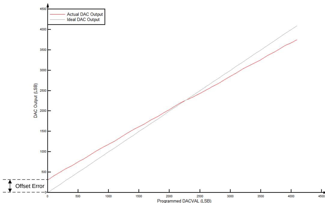
Figure 5-43. CMPSS DAC Static Offset
