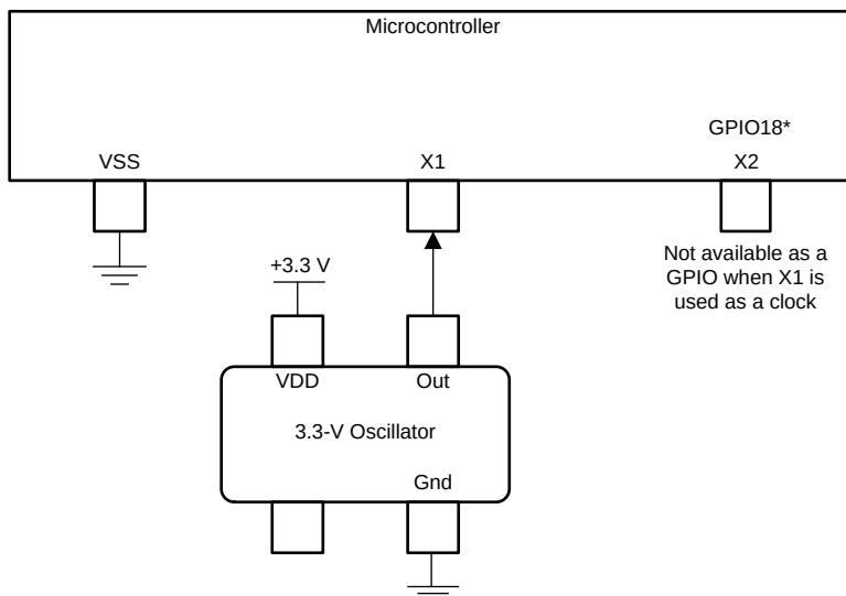
Figure 5-11. Single-ended 3.3-V External Clock
