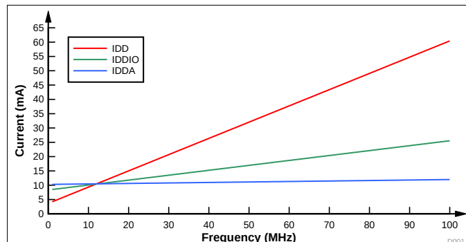
Figure 5-1. Current Versus Frequency — External Supply
