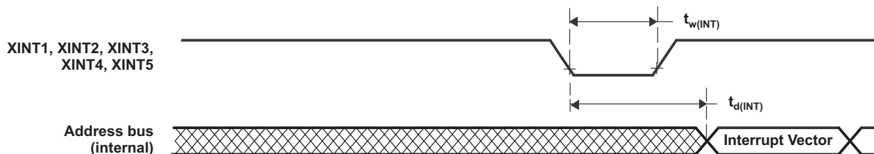
Figure 5-24. External Interrupt Timing
