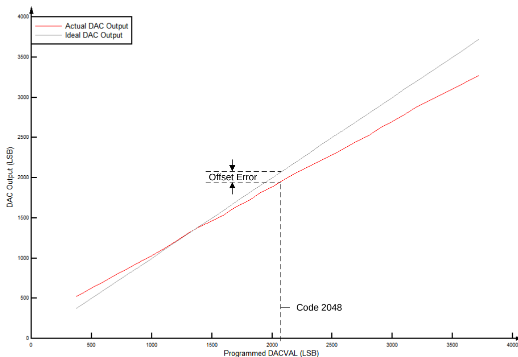
Figure 5-37. Buffered DAC Offset
