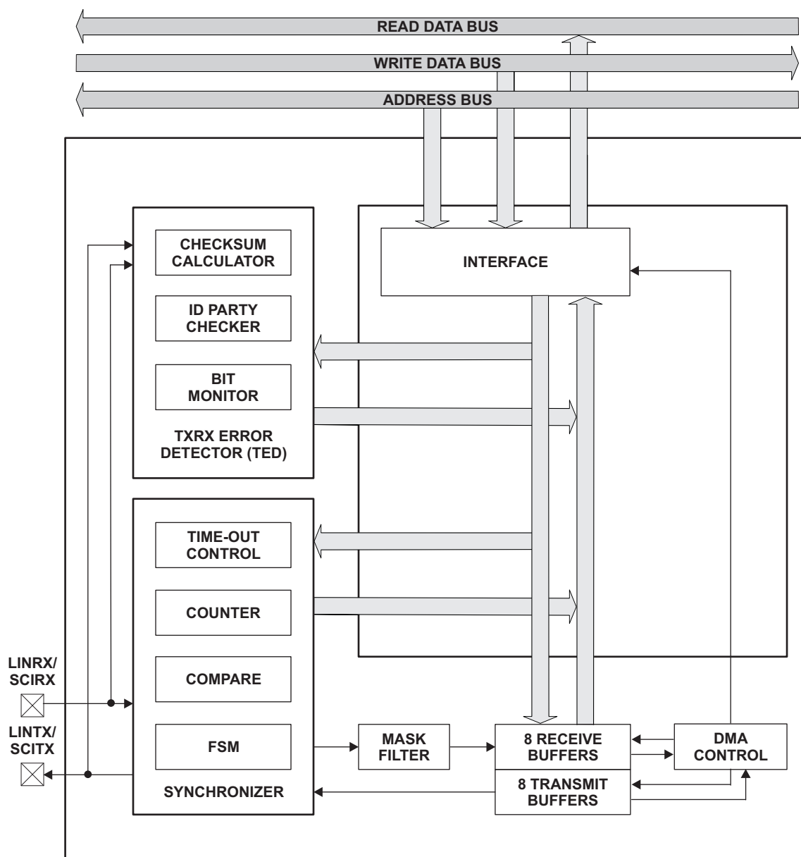
Figure 5-74. LIN Block Diagram
