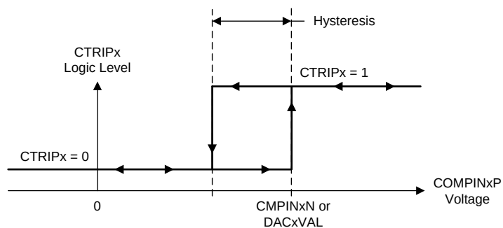
Figure 5-42. CMPSS Comparator Hysteresis
