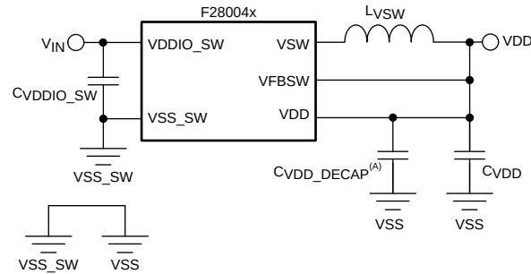
Figure 5-5. DC-DC Circuit Schematic
