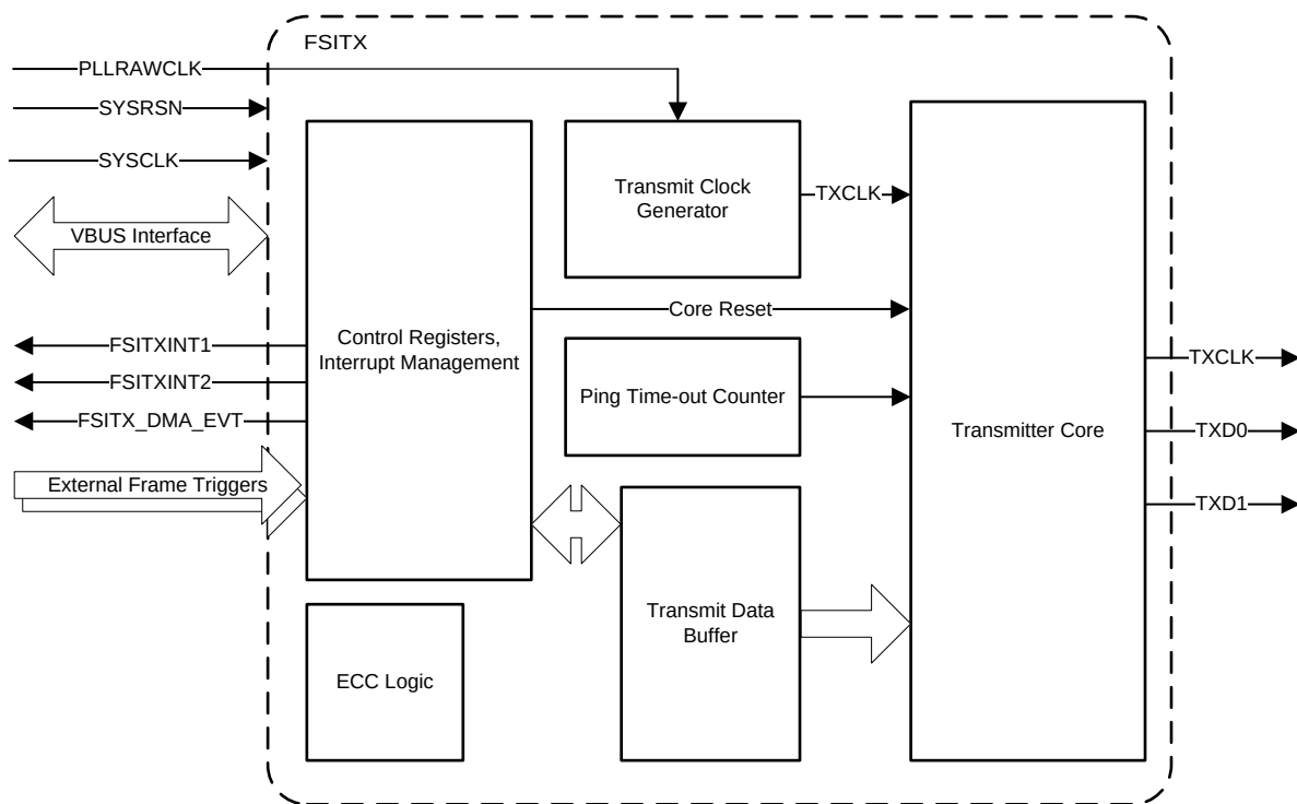
Figure 5-76. FSITX Block Diagram
