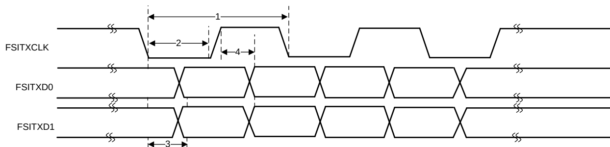
Figure 5-77. FSITX Timings
