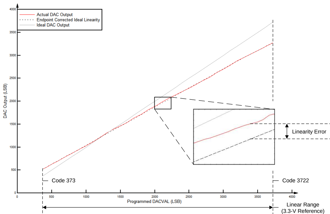
Figure 5-39. Buffered DAC Linearity
