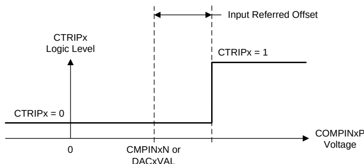
Figure 5-41. CMPSS Comparator Input Referred Offset
