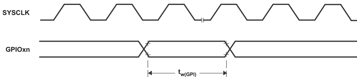
Figure 5-22. General-Purpose Input Timing
