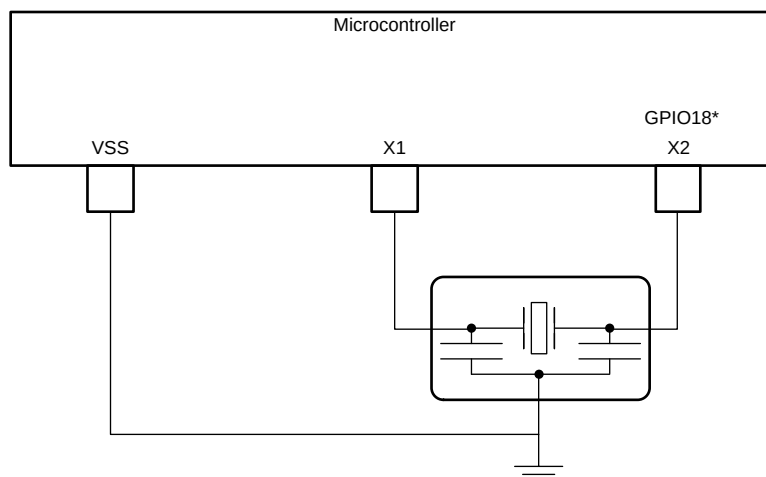
Figure 5-13. External Resonator
