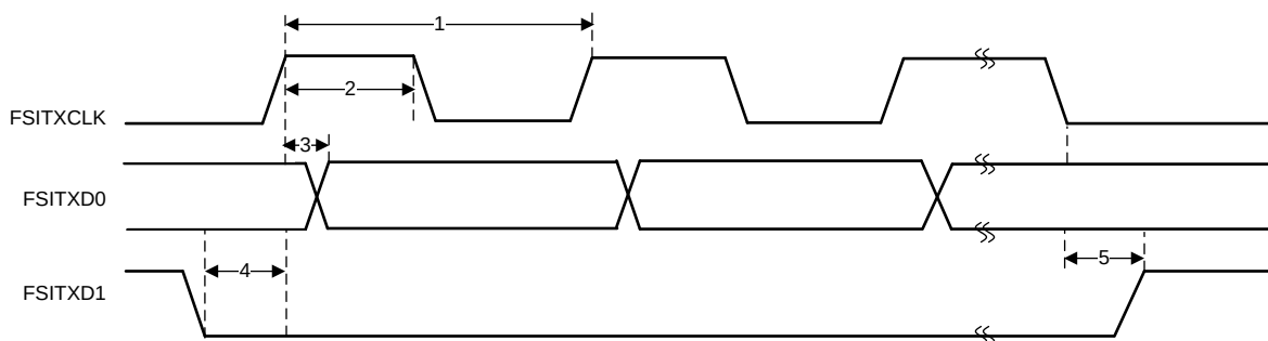
Figure 5-81. FSITX SPI Mode Timings
