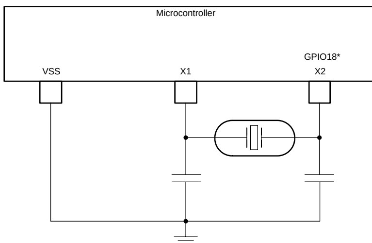
Figure 5-12. External Crystal
