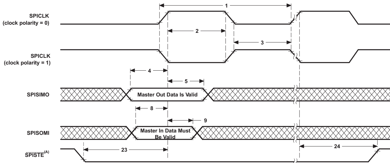
Figure 5-70. High-Speed SPI Master Mode External Timing (Clock Phase = 0)
