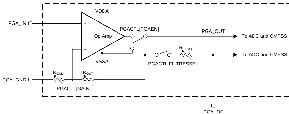
Figure 5-35. PGA Block Diagram
