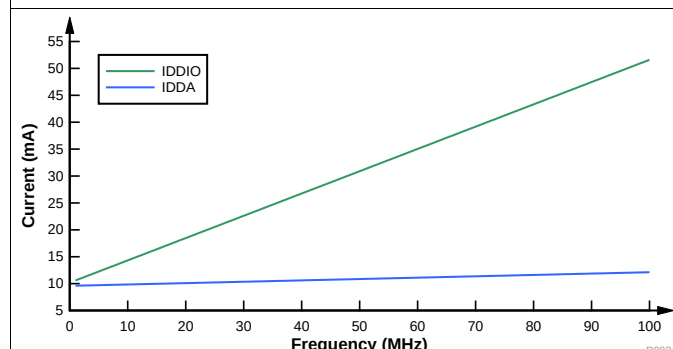
Figure 5-3. Current Versus Frequency — DCDC
