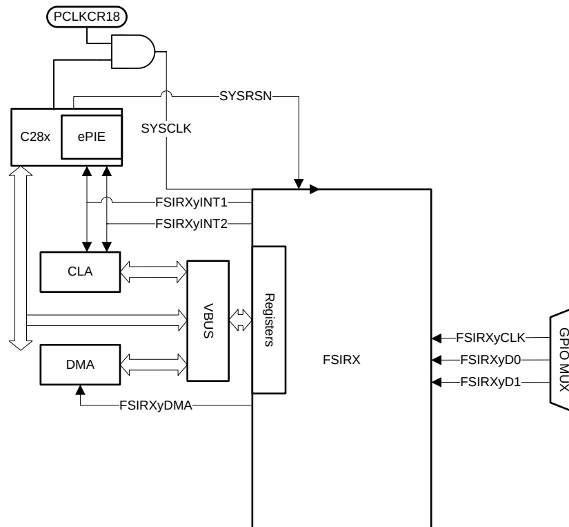
Figure 5-78. FSIRX CPU Interface
