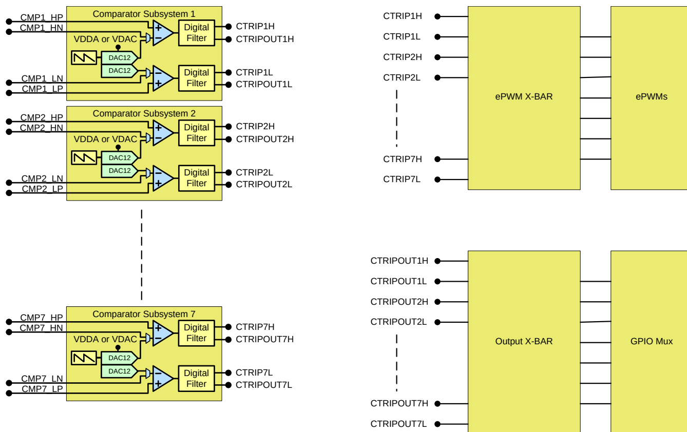
Figure 5-40. CMPSS Connectivity
