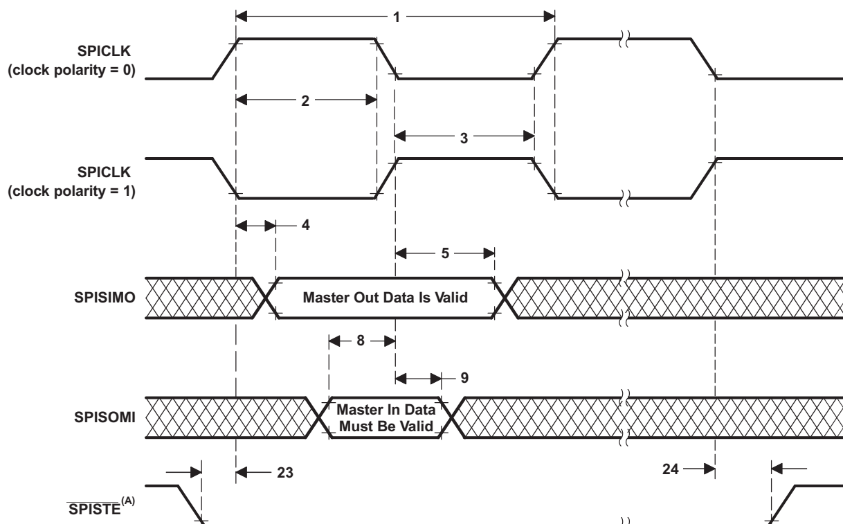
Figure 5-66. SPI Master Mode External Timing (Clock Phase = 0)
