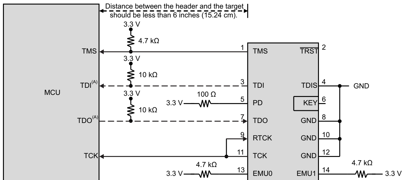
Figure 5-16. Connecting to the 14-Pin JTAG Header
