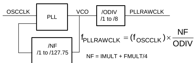
Figure 5-10. System PLL
