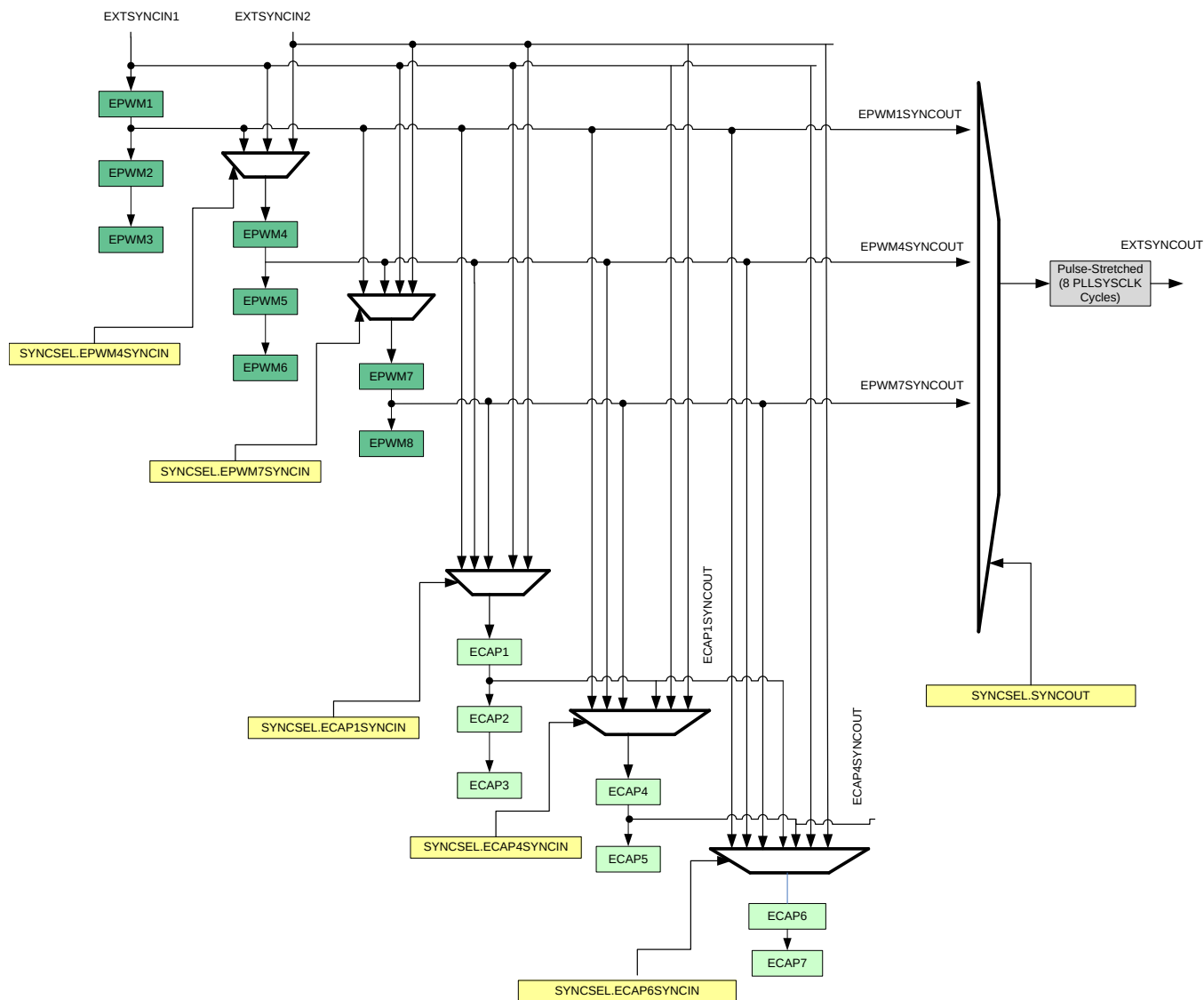
Figure 5-52. Synchronization Chain Architecture
