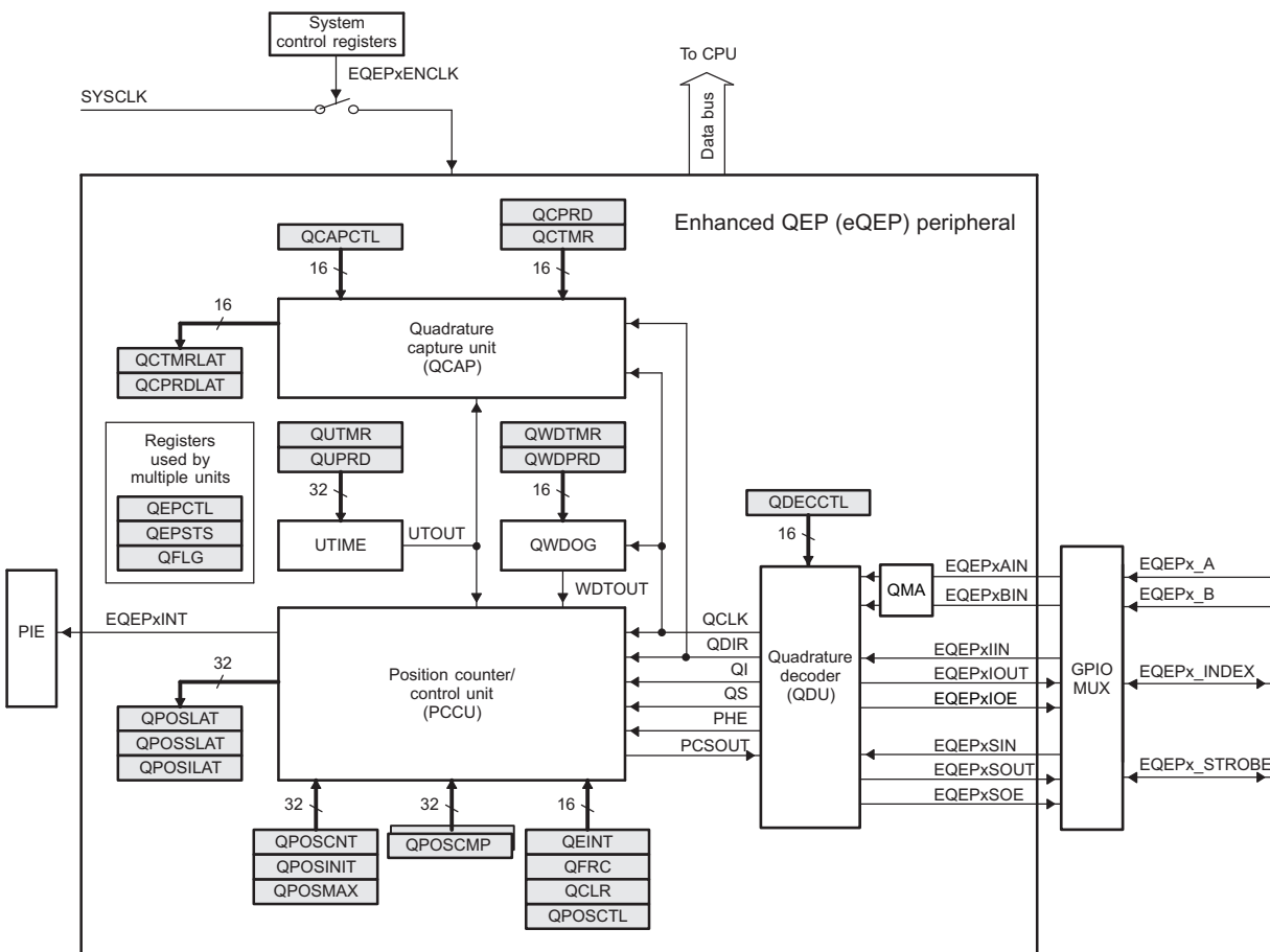
Figure 5-55. eQEP Block Diagram
