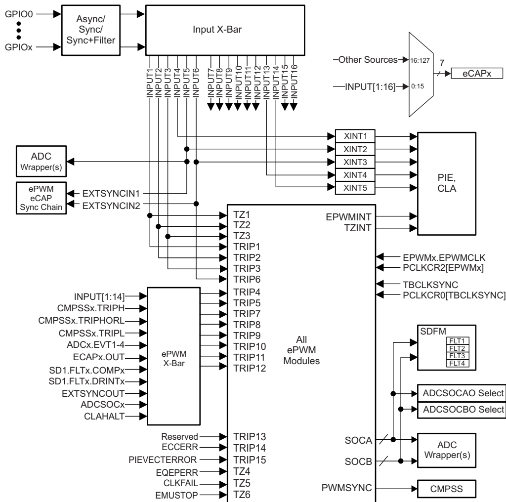
Figure 5-51. ePWM Trip Input Connectivity
