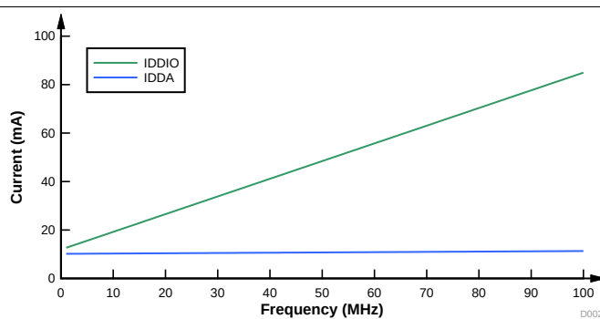
Figure 5-2. Current Versus Frequency — Internal VREG
