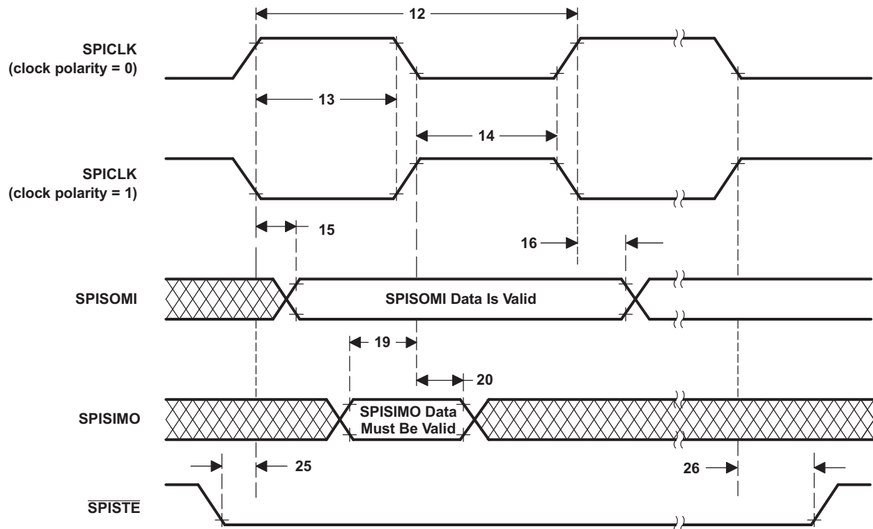
Figure 5-72. High-Speed SPI Slave Mode External Timing (Clock Phase = 0)
