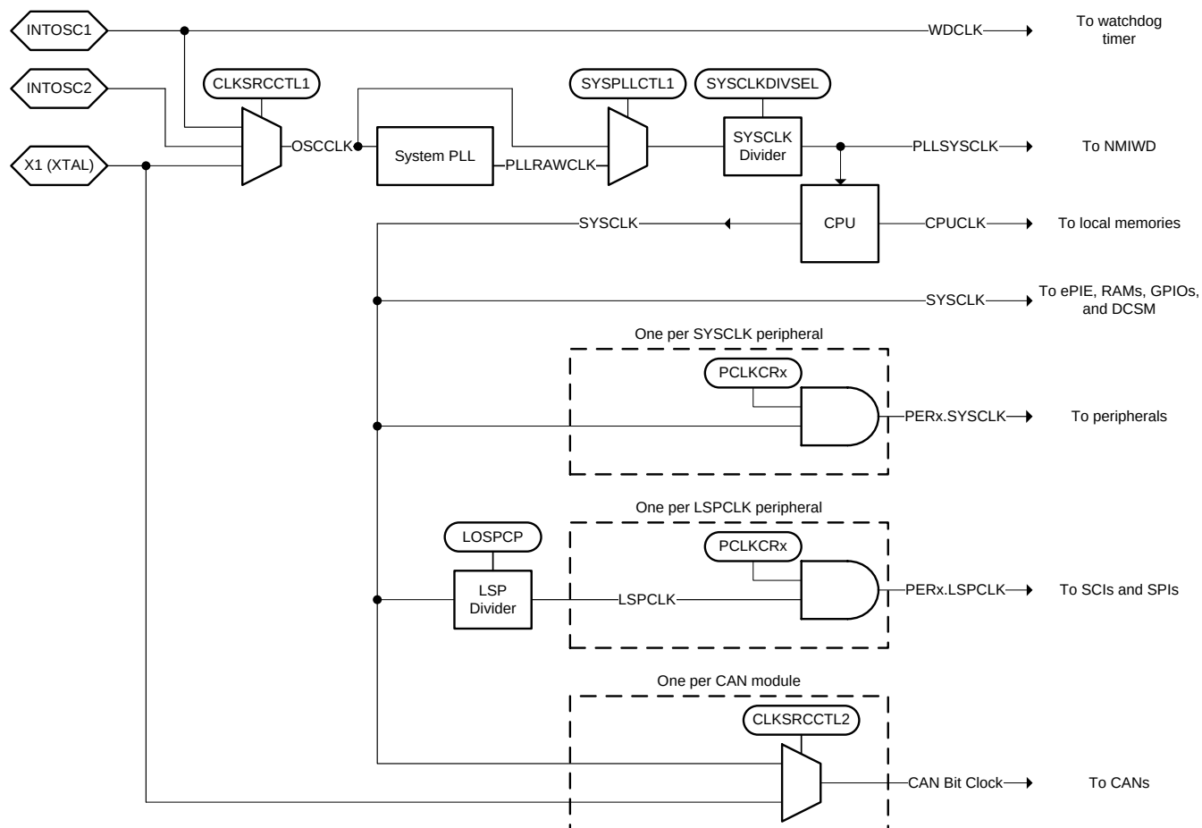
Figure 5-9. Clocking System
