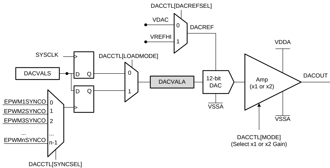
Figure 5-36. DAC Module Block Diagram
