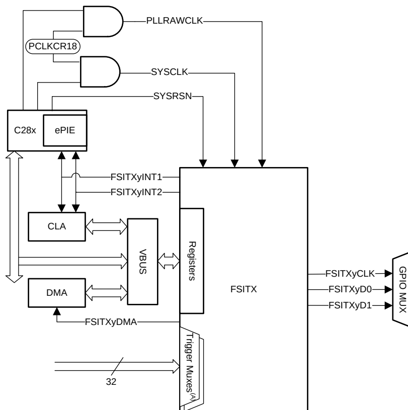
Figure 5-75. FSITX CPU Interface
