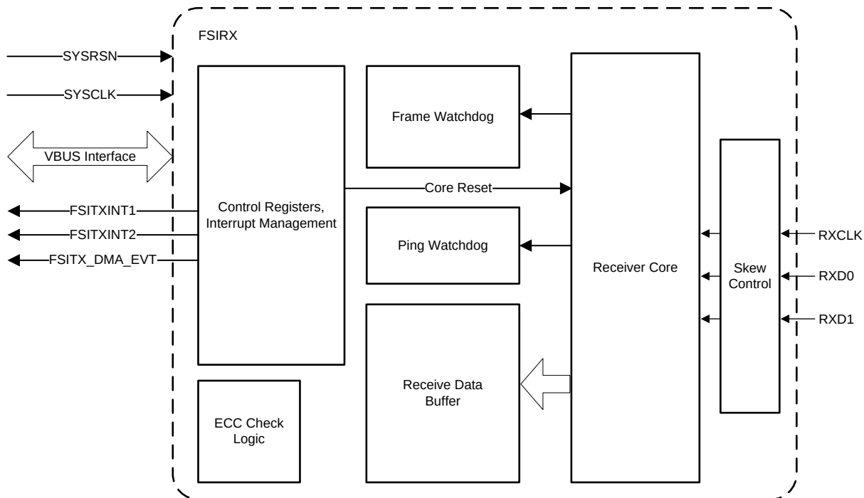
Figure 5-79. FSIRX Block Diagram
