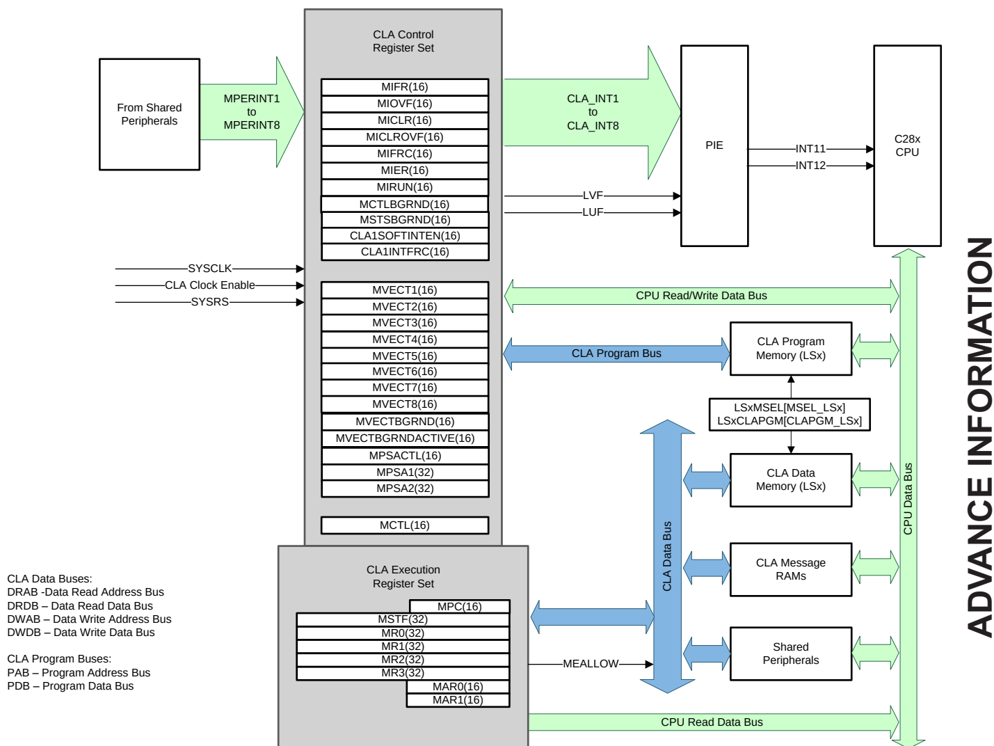
Figure 6-2. CLA Block Diagram
