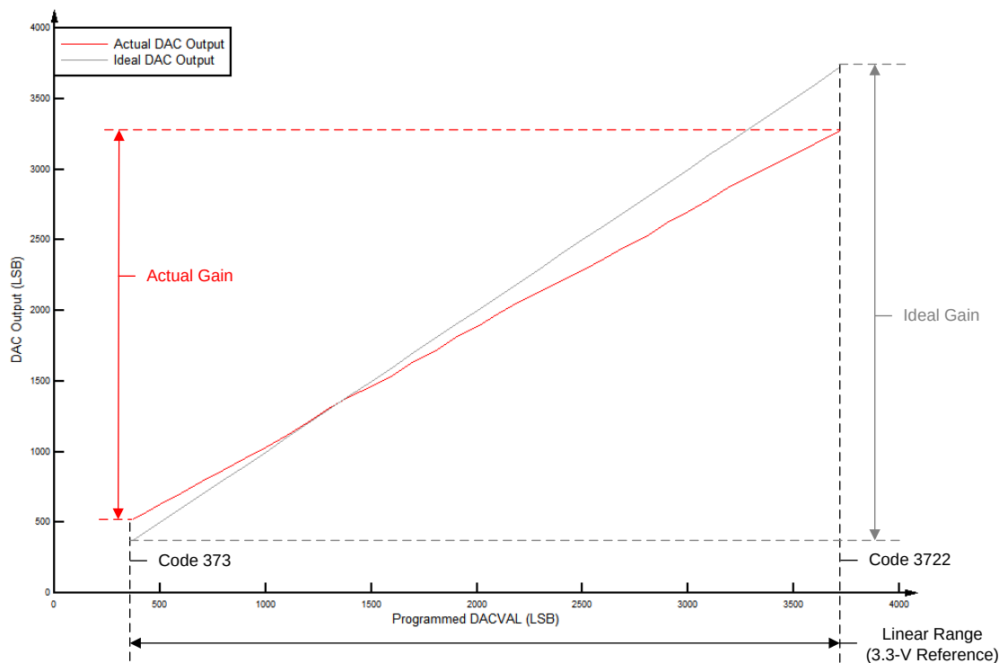
Figure 5-38. Buffered DAC Gain
