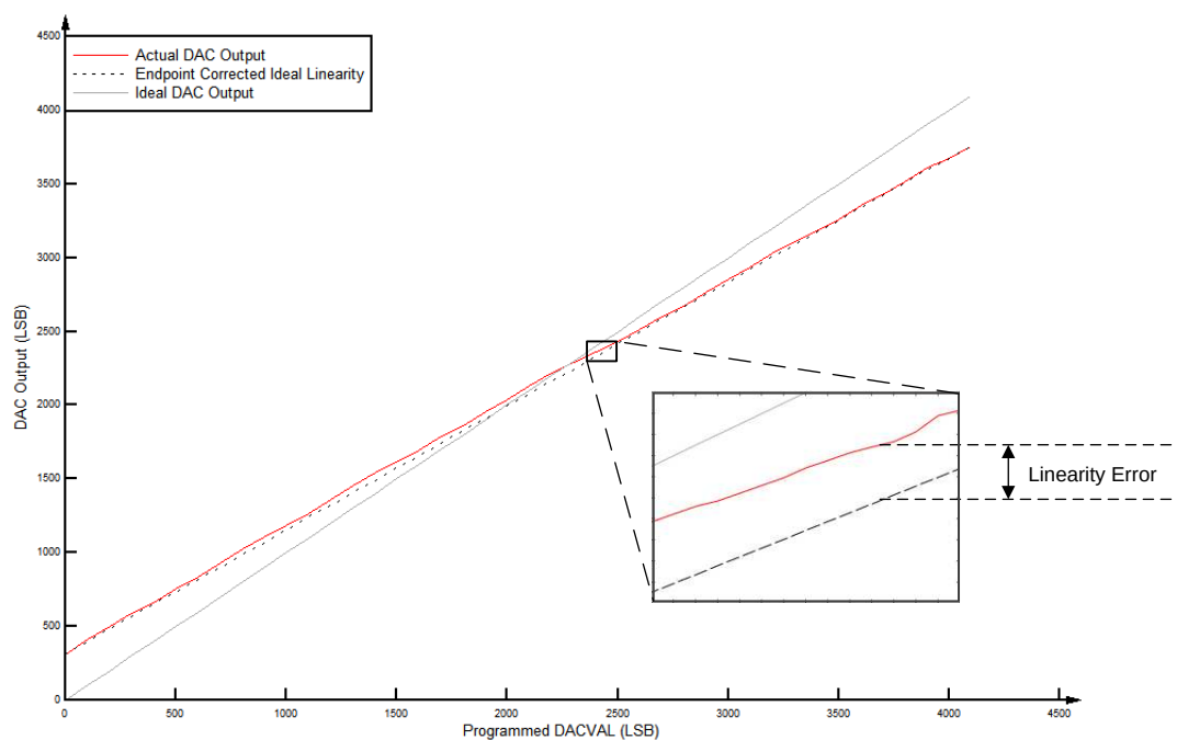
Figure 5-45. CMPSS DAC Static Linearity
