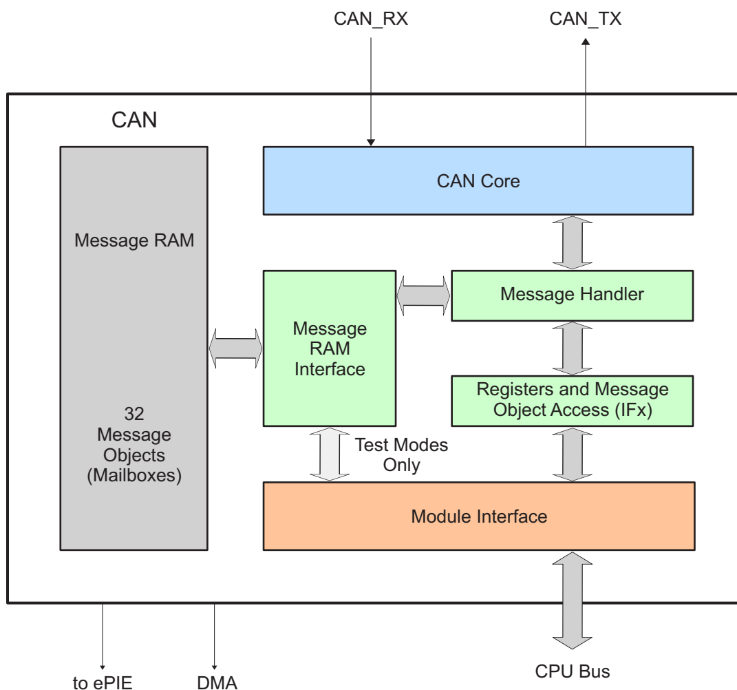
Figure 5-61. CAN Block Diagram
