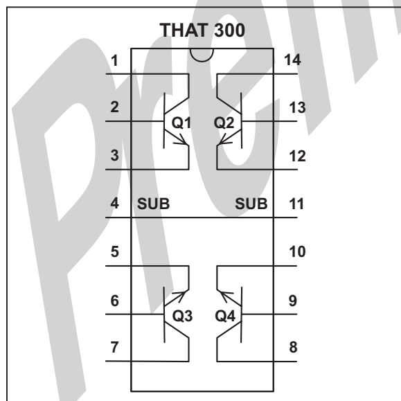
Fig 1. 300 Pinout
