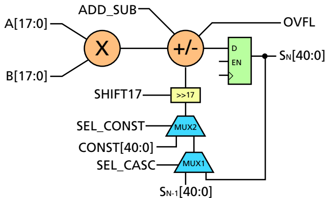
Figure 1-1 • RTAX-DSP Mathblock
