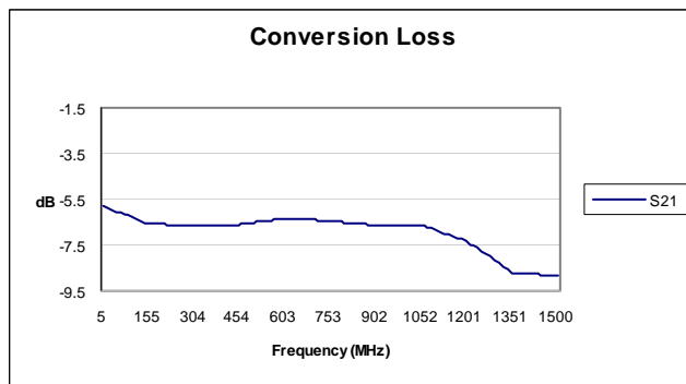
Typical Test Data – Conversion Loss
